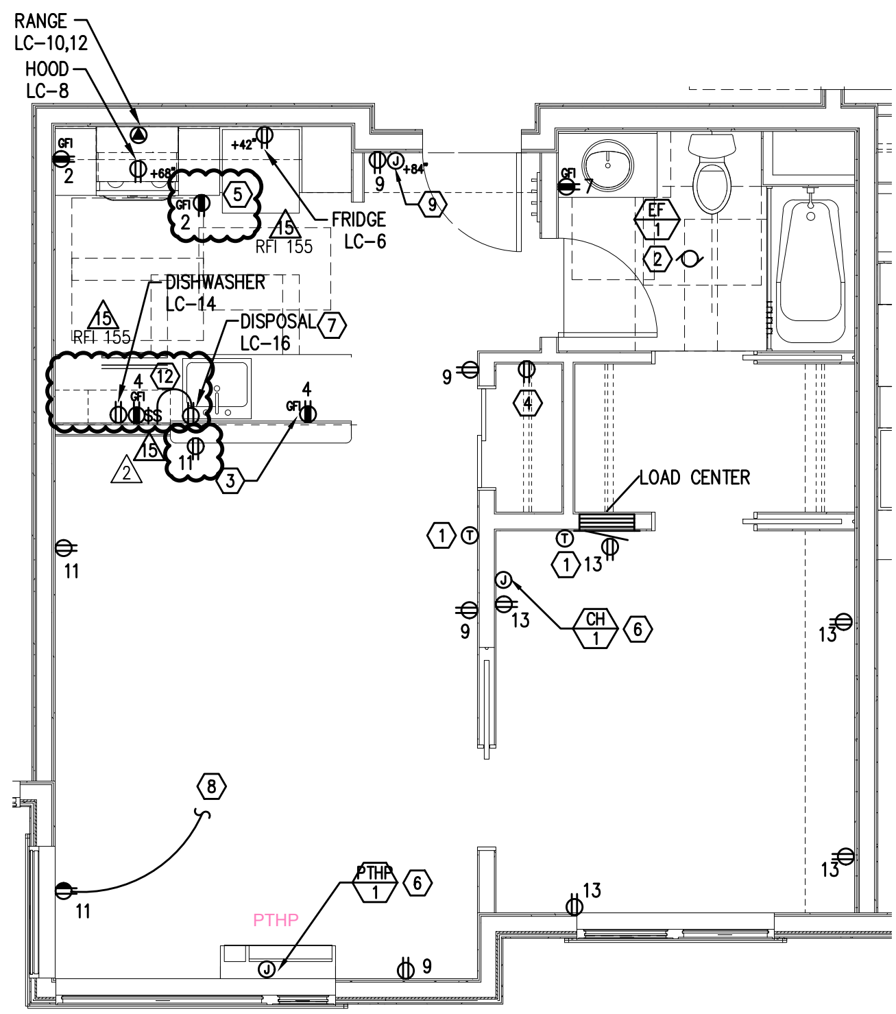
4 E4.13 TYPICAL UNIT TYPE 1C - POWER PLAN SCALE: 1/4" = 1'-0" (FLOORS 2-6)
