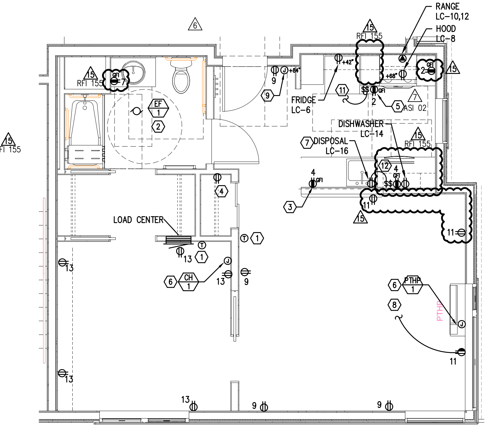
1 E4.13 TYPICAL UNIT TYPE 1A ADA - POWER PLAN SCALE: 1/4" = 1'-0" (UNIT 209) NOTE: UNIT 209 IS ADA/FHA TYPE A. INCLUDE STROBES WITH FIRE ALARMS AND VISUAL DOORBELL SIGNAL PER ADAS 809.5. ASI 02
