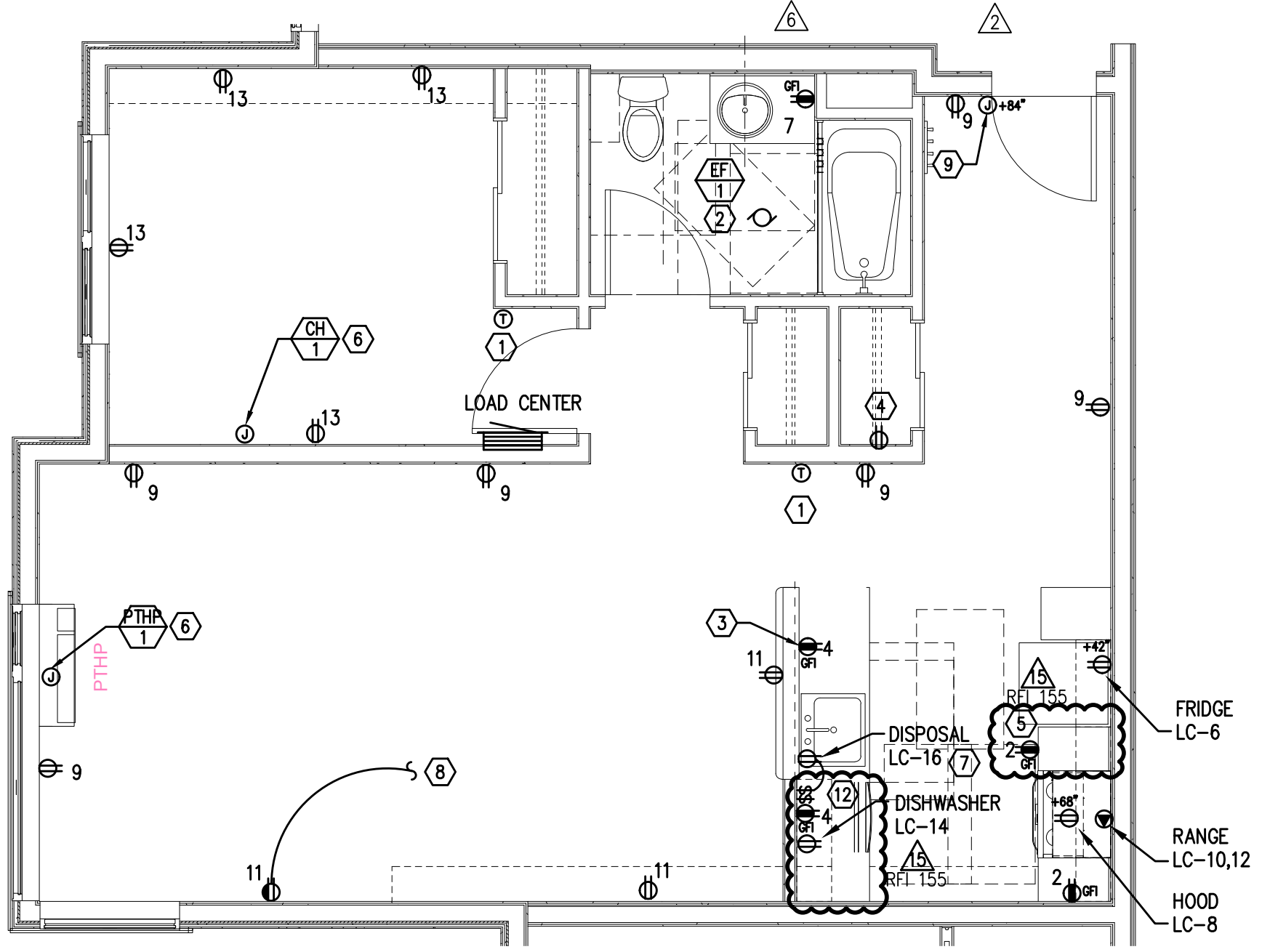
3 E4.13 TYPICAL UNIT TYPE 1B - POWER PLAN SCALE: 1/4" = 1'-0" (FLOORS 2-6)
