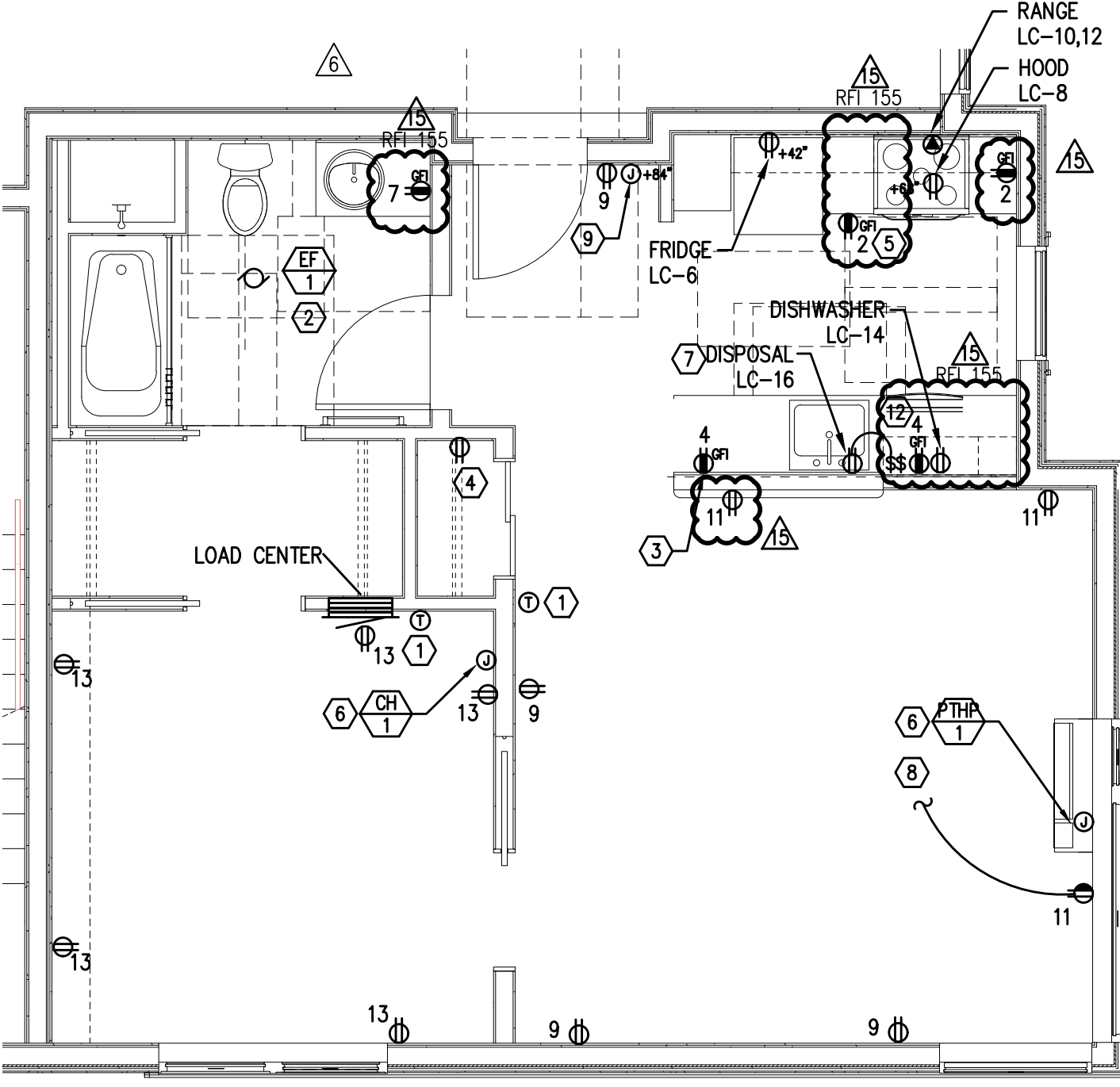
2 E4.13 TYPICAL UNIT TYPE 1A - POWER PLAN SCALE: 1/4" = 1'-0" (FLOORS 3-6)
