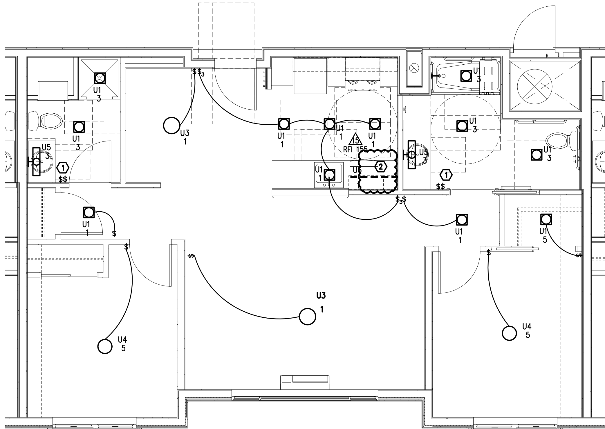
2 TYPICAL UNIT TYPE 2A/ADA - LIGHTING PLAN SCALE: 1/4" = 1'-0" (UNITS 411,511,611)
