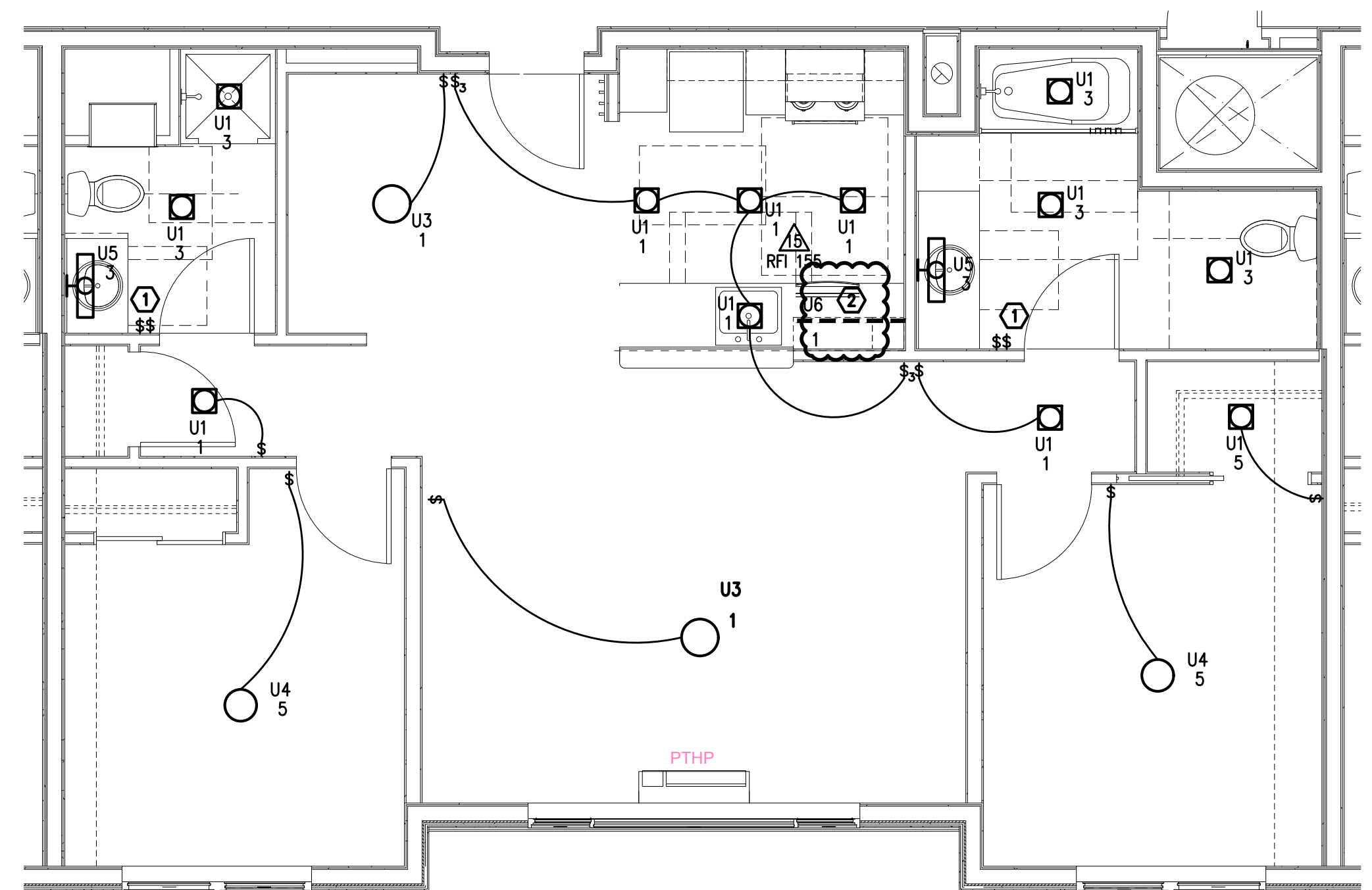
3 TYPICAL UNIT TYPE 2A - LIGHTING PLAN SCALE: 1/4" = 1'-0" (UNITS 211,311)
