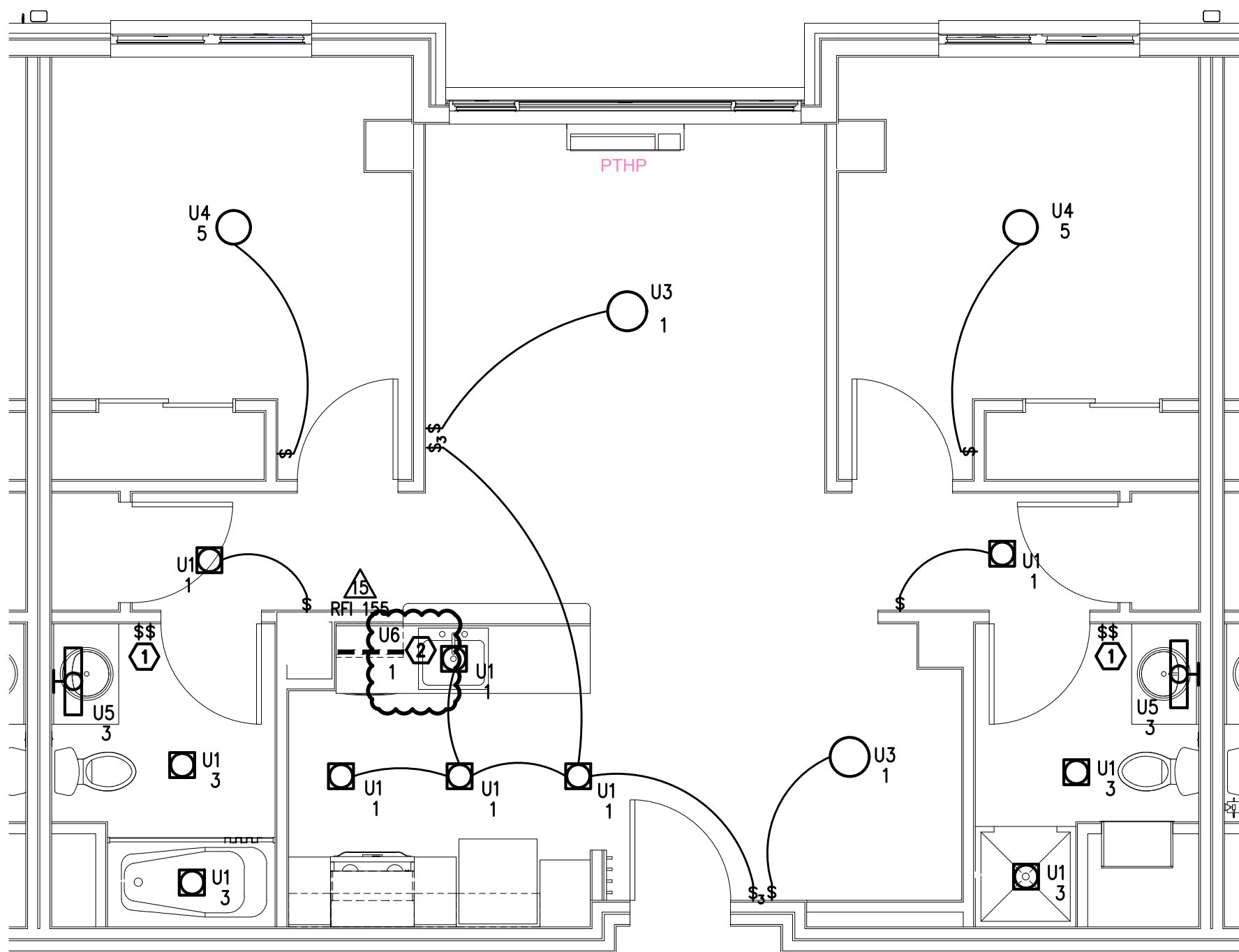
2 E4.02 TYPICAL UNIT TYPE 2B – LIGHTING PLAN SCALE: 1/4" = 1'-0"
