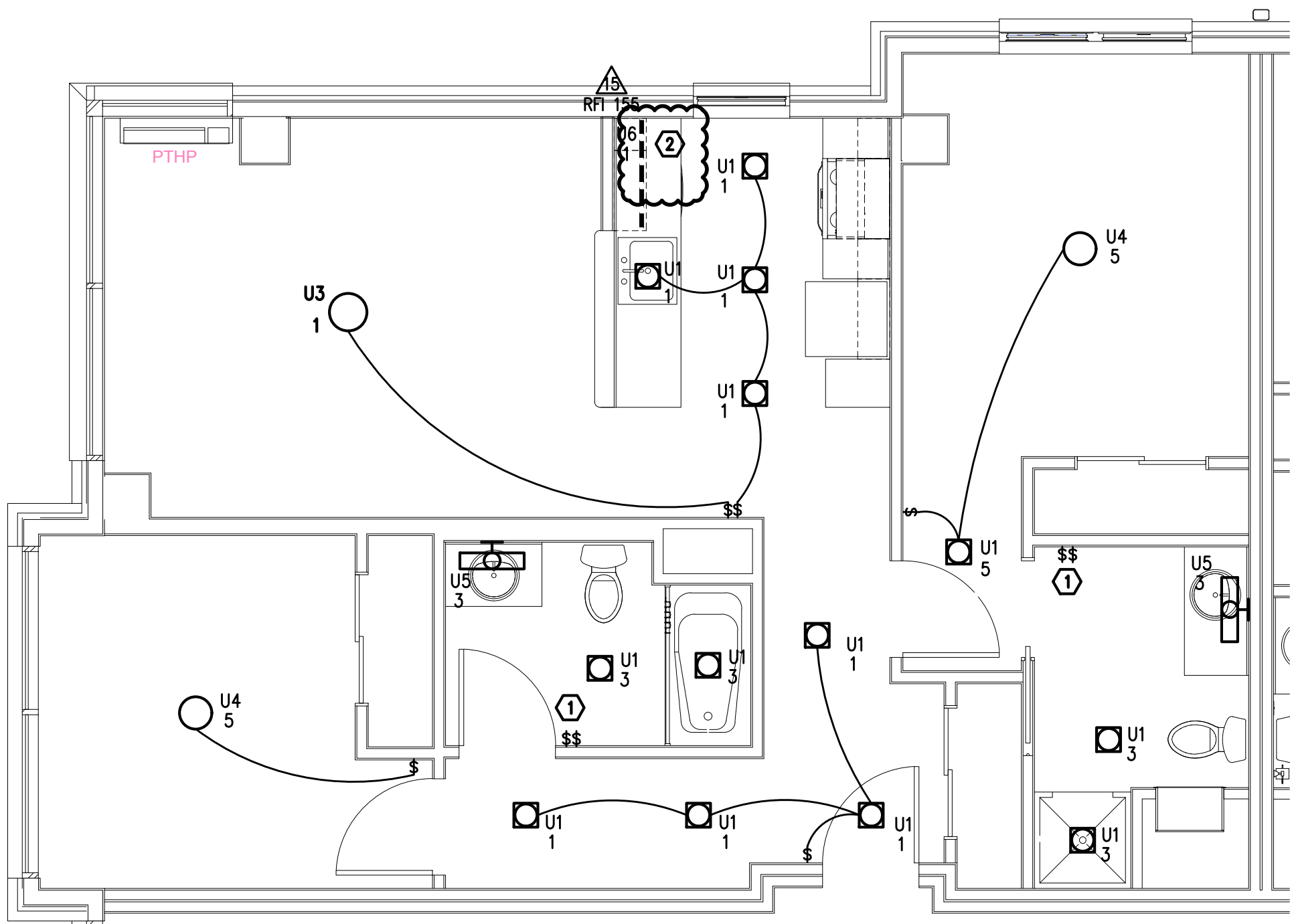
1 E4.02 TYPICAL UNIT TYPE 2A – LIGHTING PLAN SCALE: 1/4" = 1'-0"
