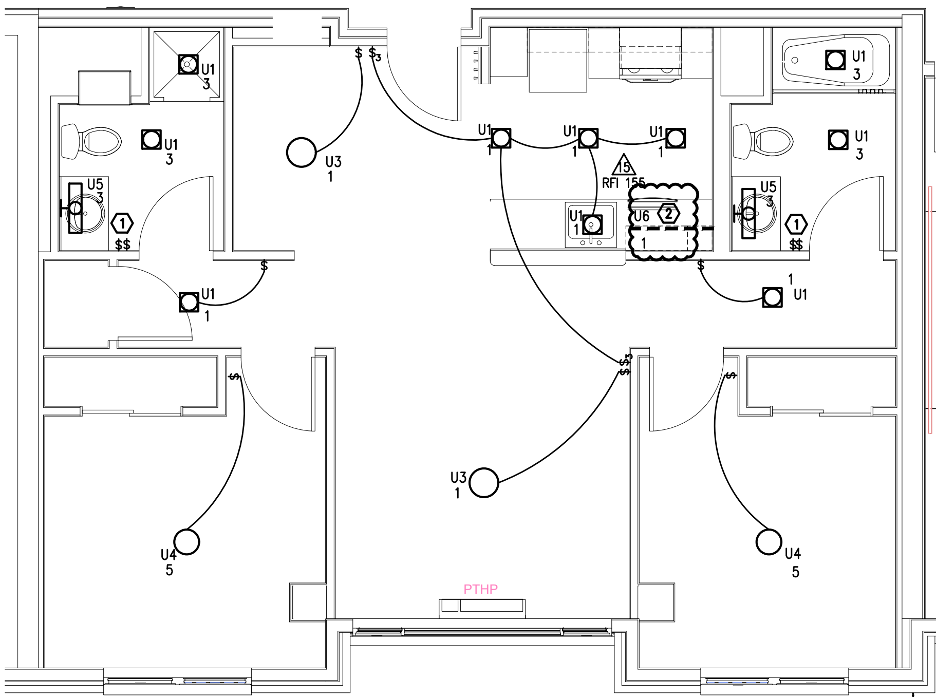
3 E4.02 TYPICAL UNIT TYPE 2C – LIGHTING PLAN SCALE: 1/4" = 1'-0"
