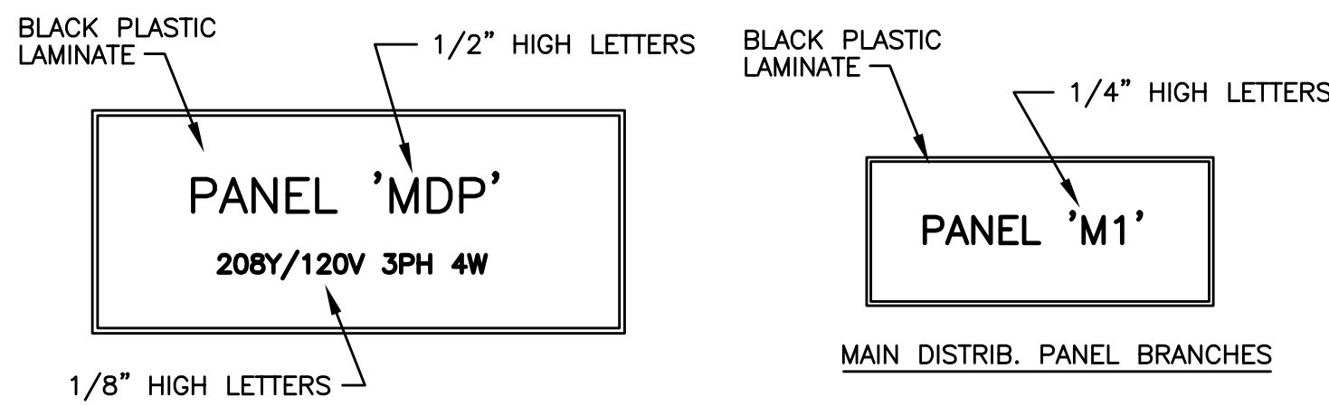
MAIN DISTRIB. PANEL LABELING
