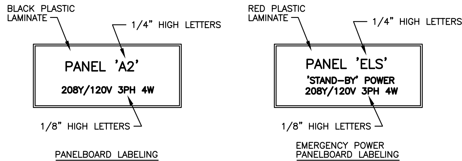
PANELBOARD LABELING
