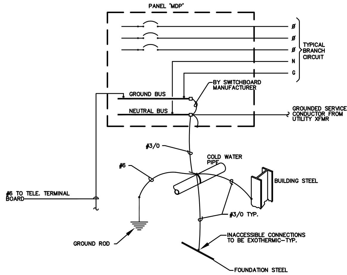
1 GROUNDING/BONDING DIAGRAM E1.23 208Y/120V, 3Ø, 4 WIRE
