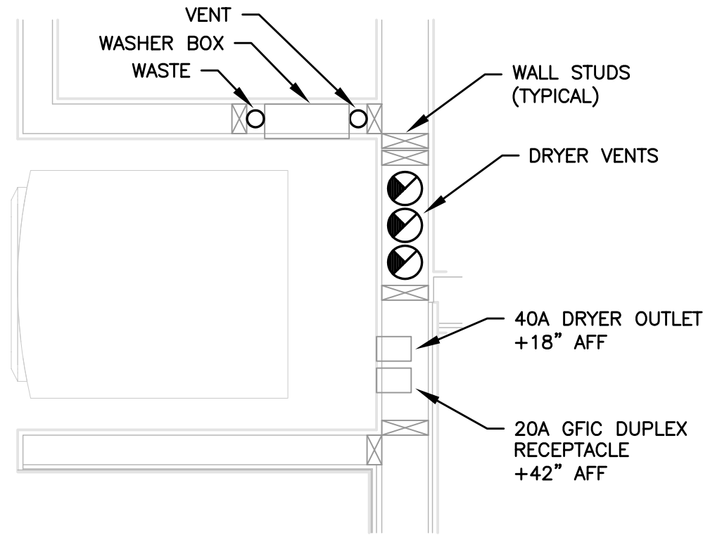
4 TYPICAL WASHER/DRYER ALCOVE E1.23 NO SCALE
