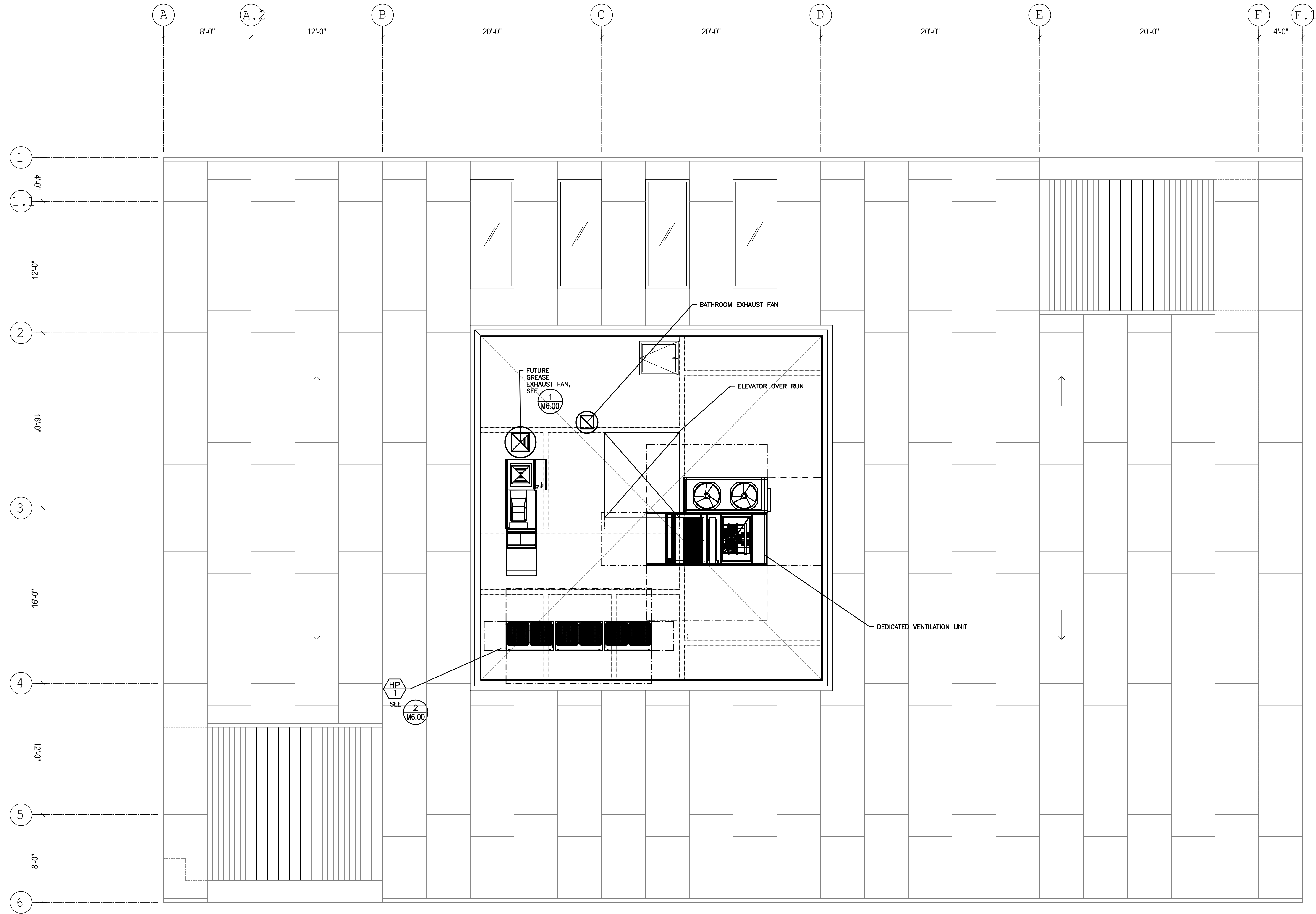
1 HVAC ROOF PLAN SCALE: 1/4" = 1'-0"
