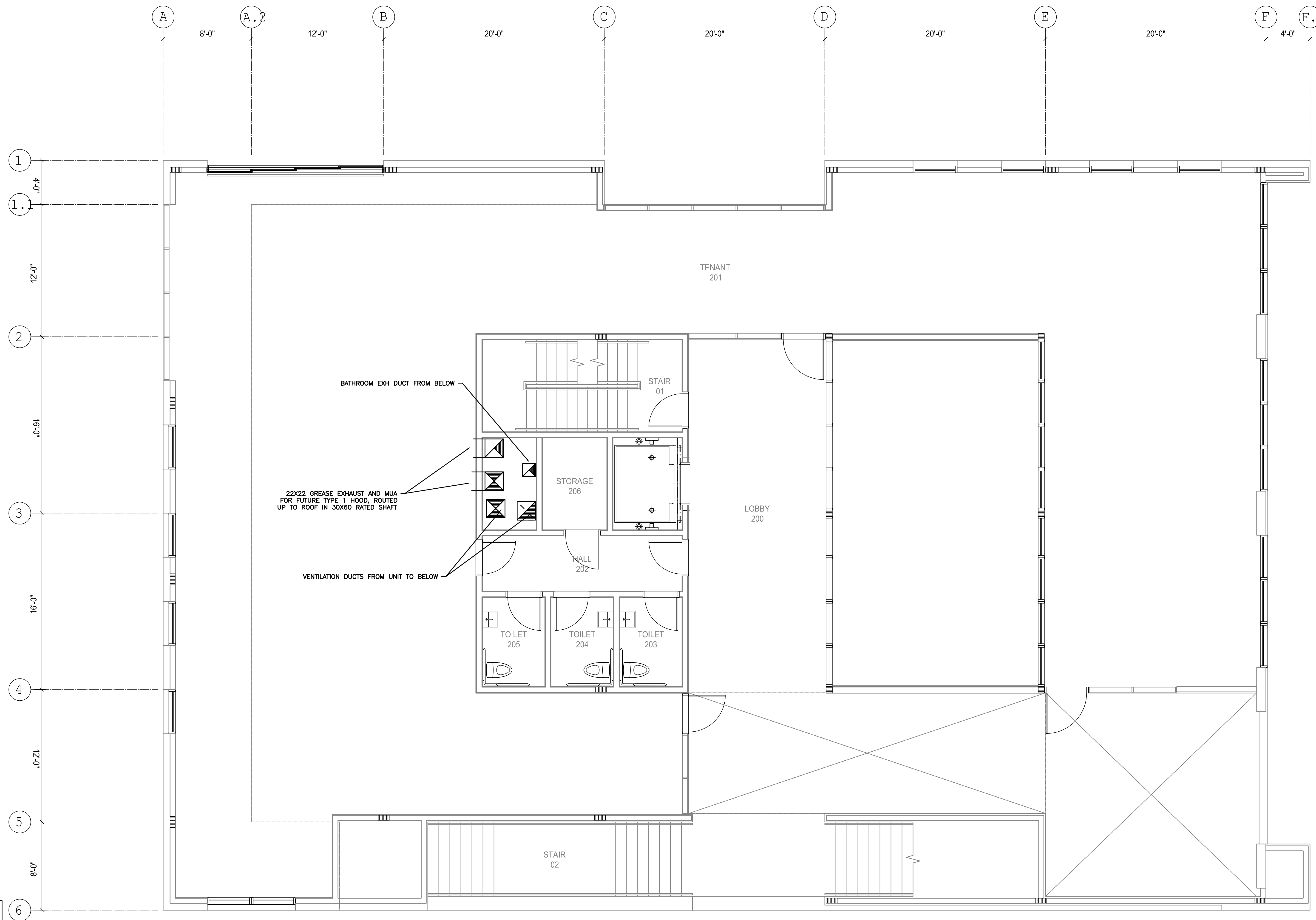
1 2ND FLOOR HVAC PLAN M2.01 SCALE: 1/4" = 1'-0"
