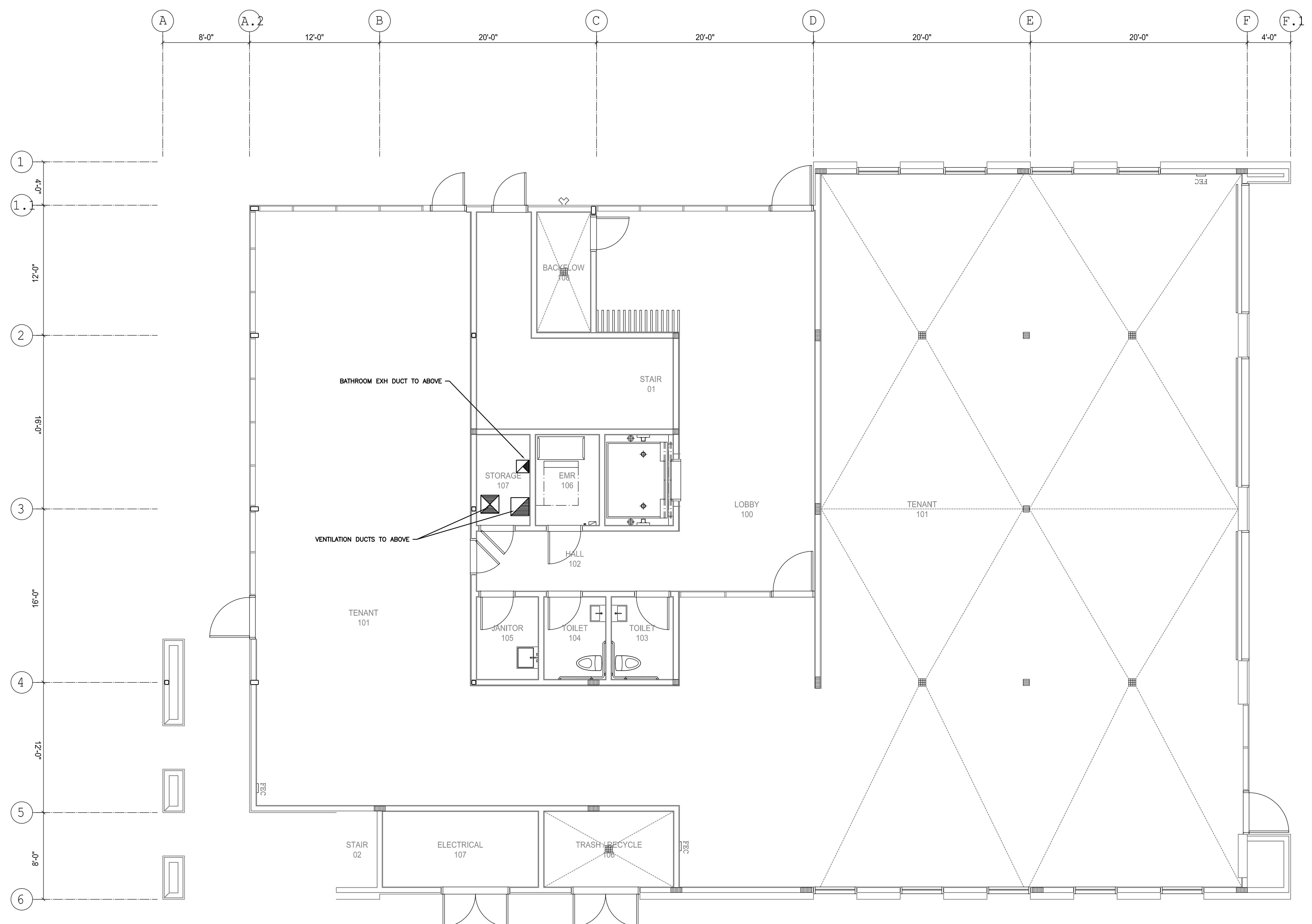
1 1st FLOOR HVAC PLAN M2.00 SCALE: 1/4" = 1'-0"
