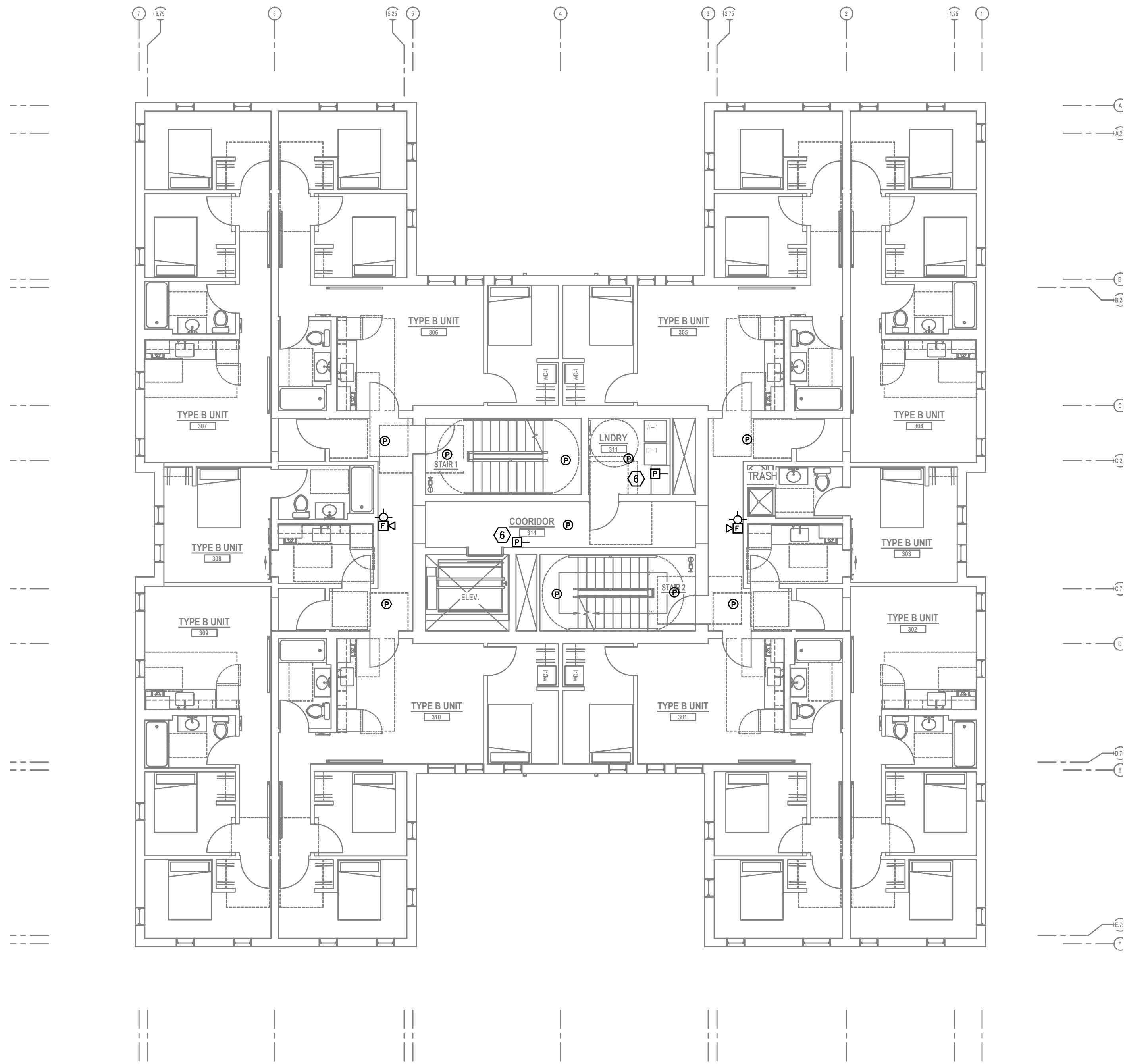
1 THIRD FLOOR TECHNOLOGY PLAN T3.03 SCALE: 1/8" = 1'-0"
