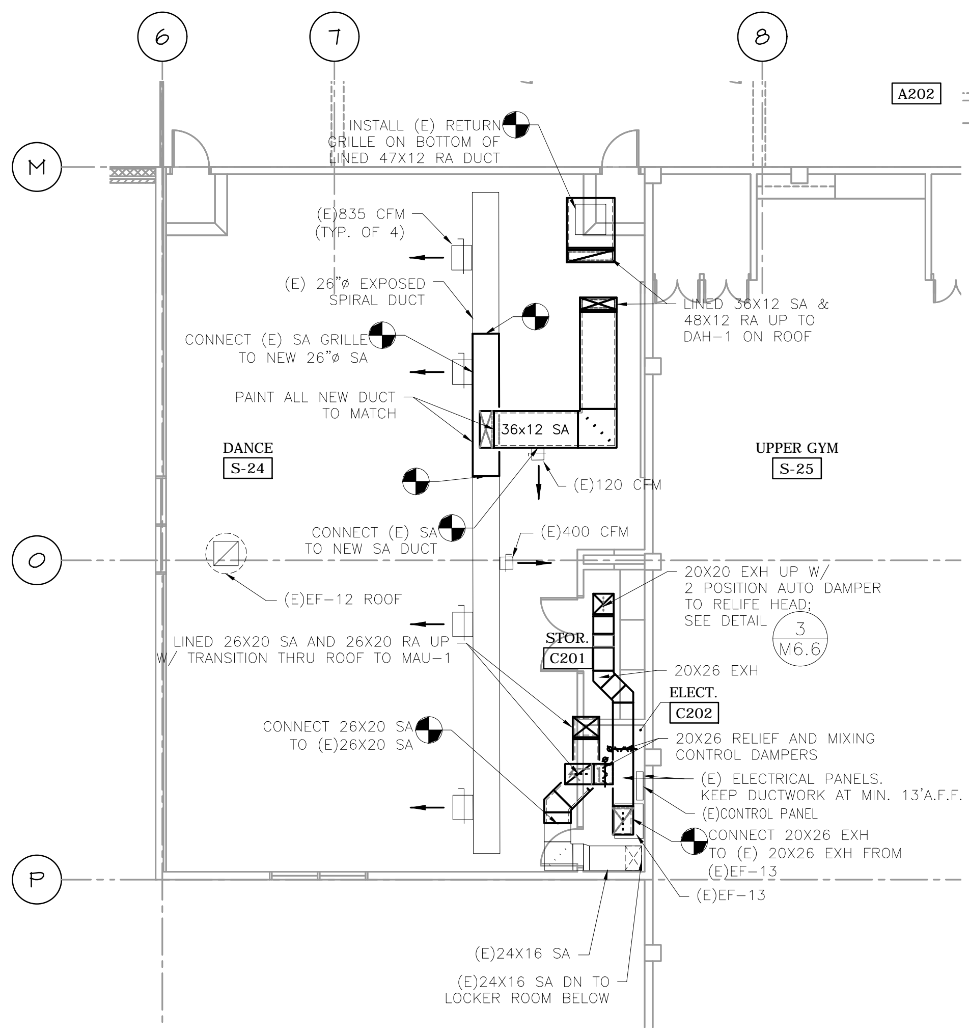
3 PARTIAL SECOND FLOOR HVAC PLAN M1.6 SCALE: 1/8"=1'-0"
