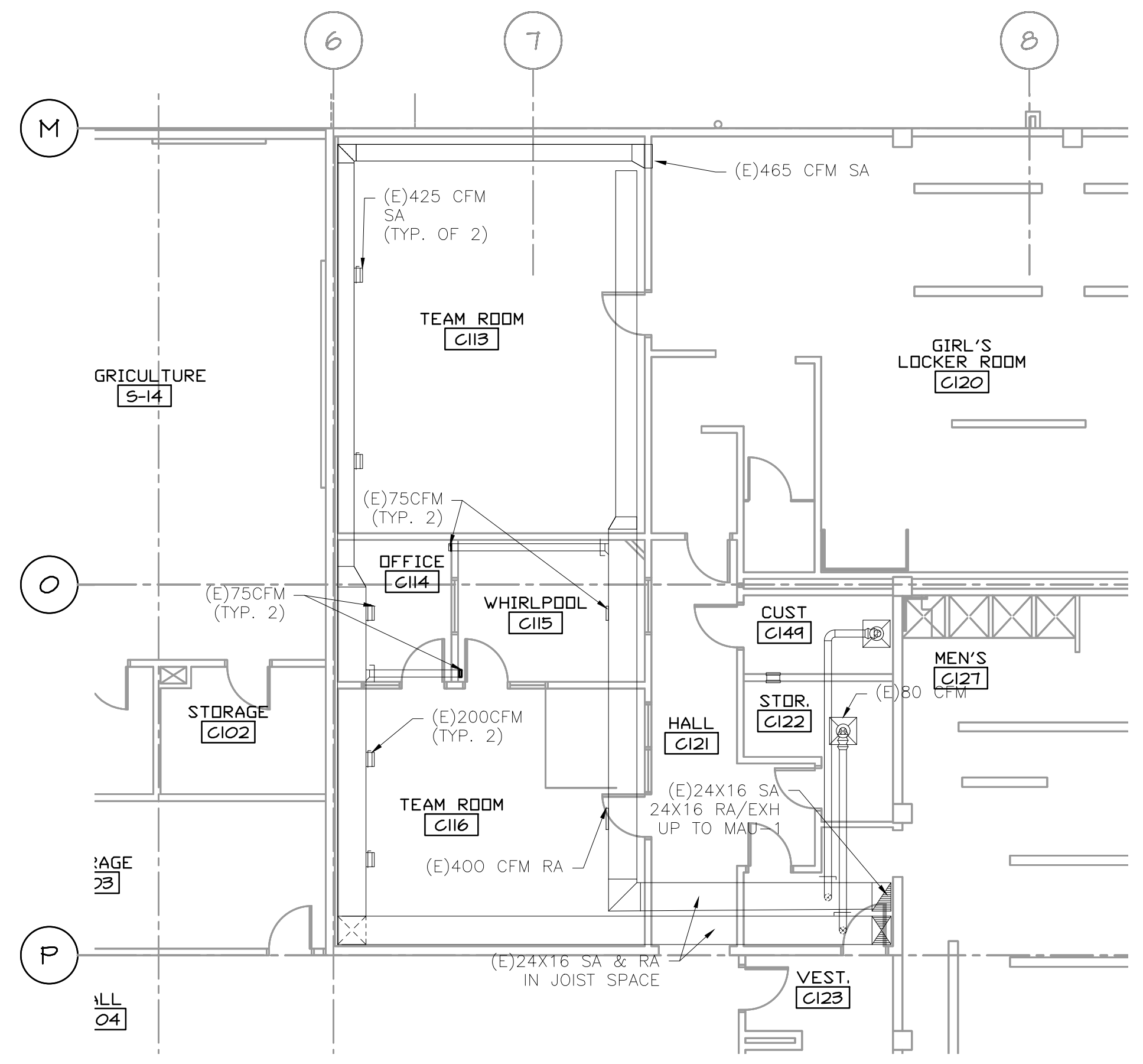
2 PARTIAL FIRST FLOOR HVAC PLAN M1.6 SCALE: 1/8"=1'-0"
