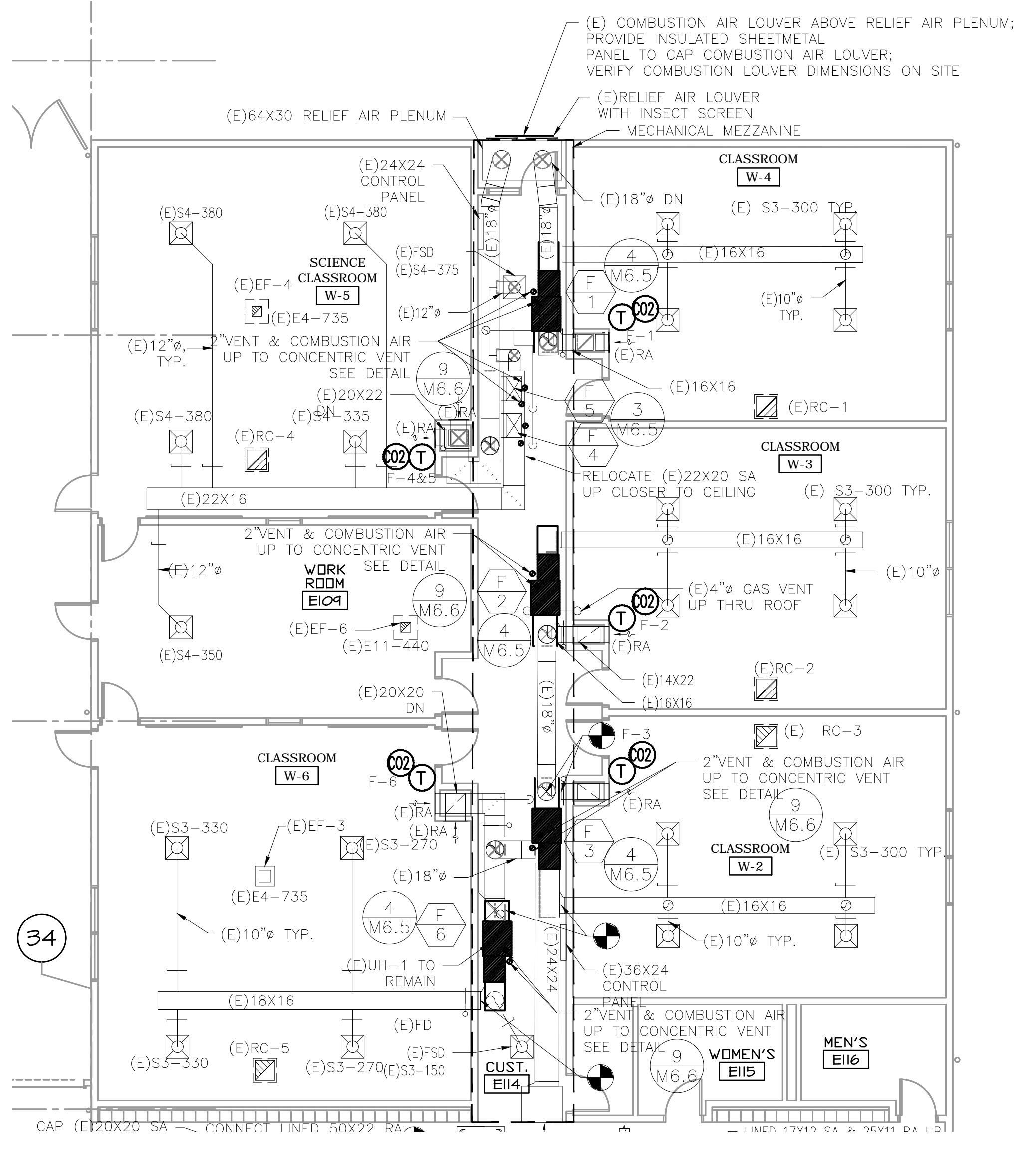
1 HVAC PARTIAL FLOOR PLAN M1.6 SCALE: 1/8"=1'-0"
