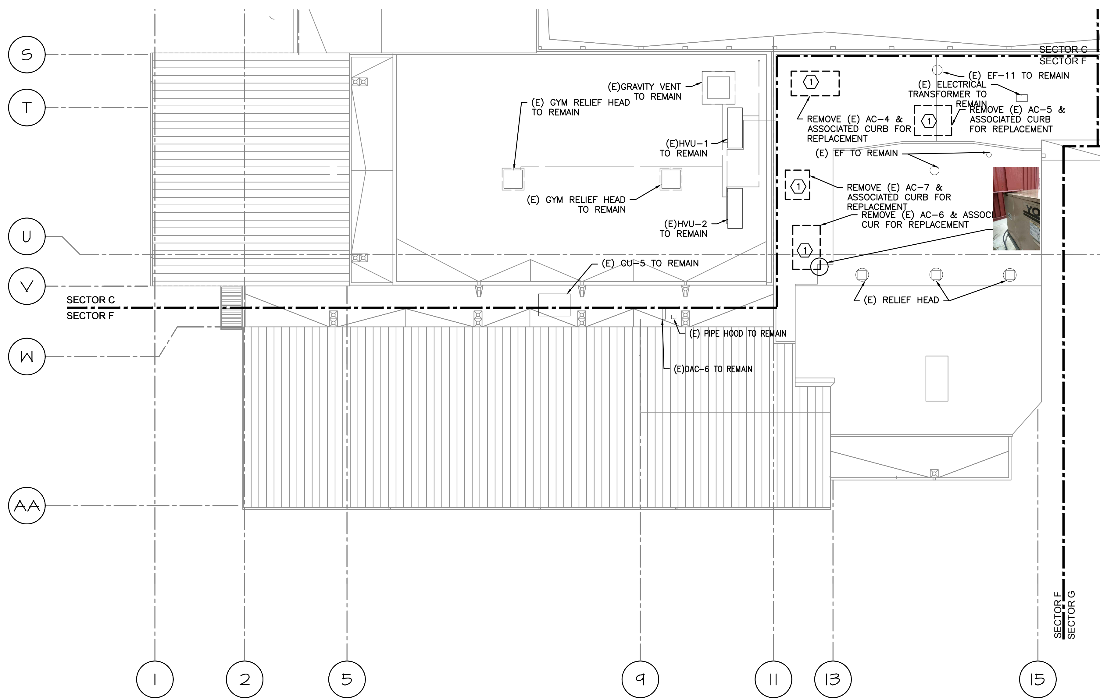
1 HVAC ROOF DEMO PLAN-SECTOR F DM2.6 SCALE: 1/16" = 1'-0"
