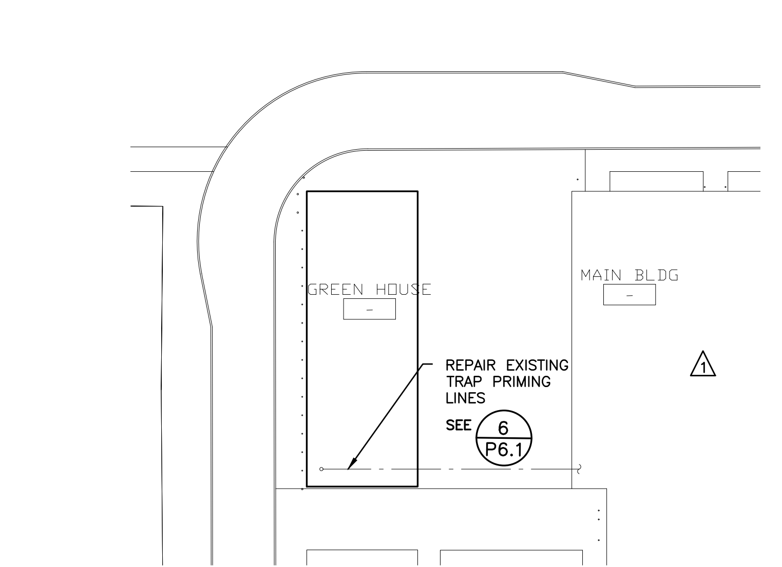
2 GREEN HOUSE SCALE: 1/16"=1'-0"
