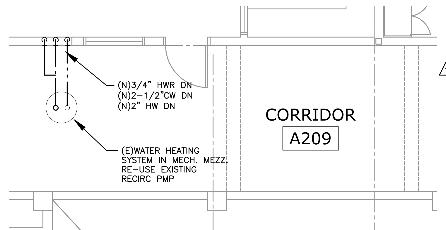
3 MECHANICAL MEZZANINE SCALE: 1/16"=1'-0"
