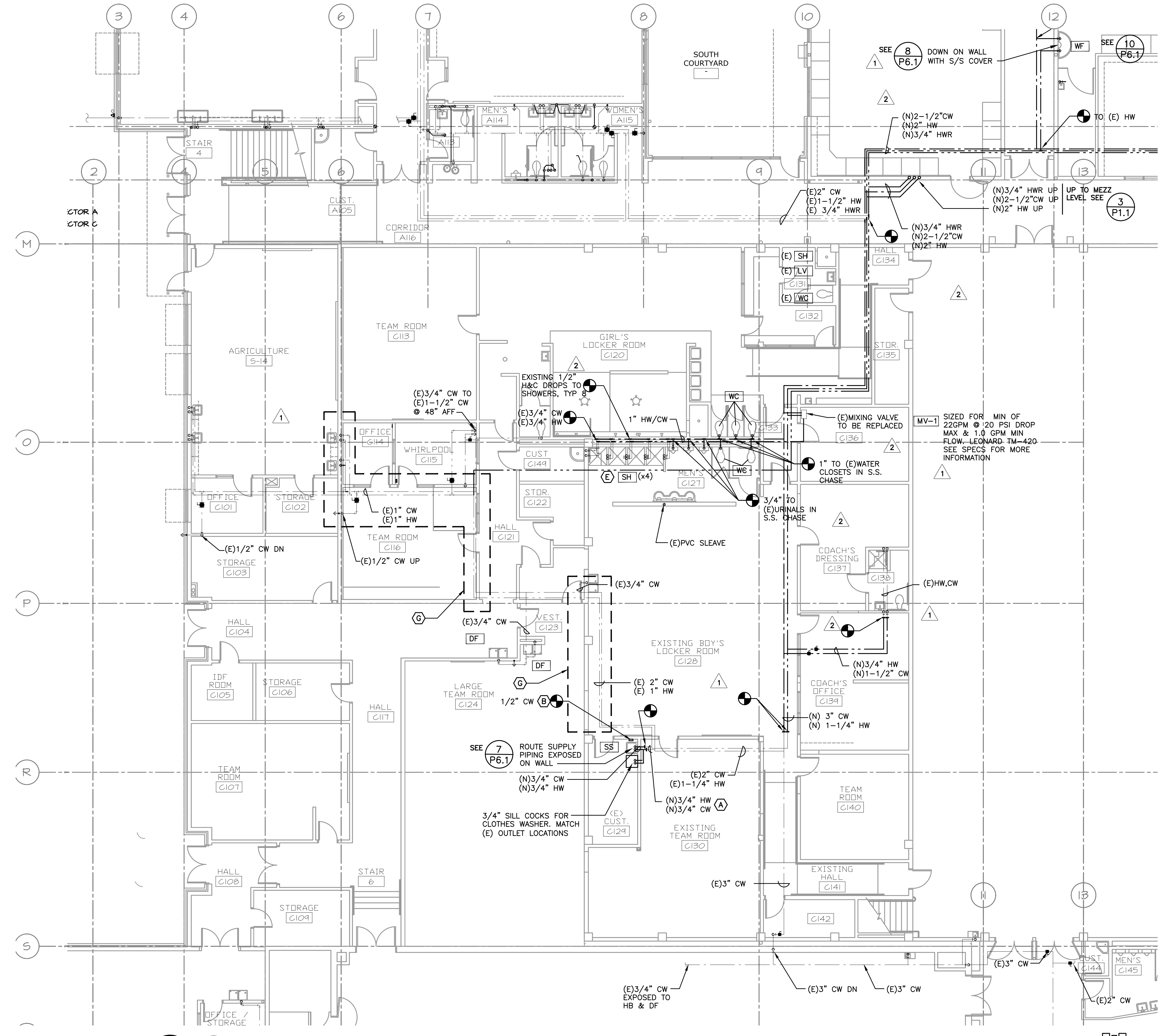
1 PARTIAL FLOOR PLUMBING PLAN SCALE: 1/8"=1'-0"
