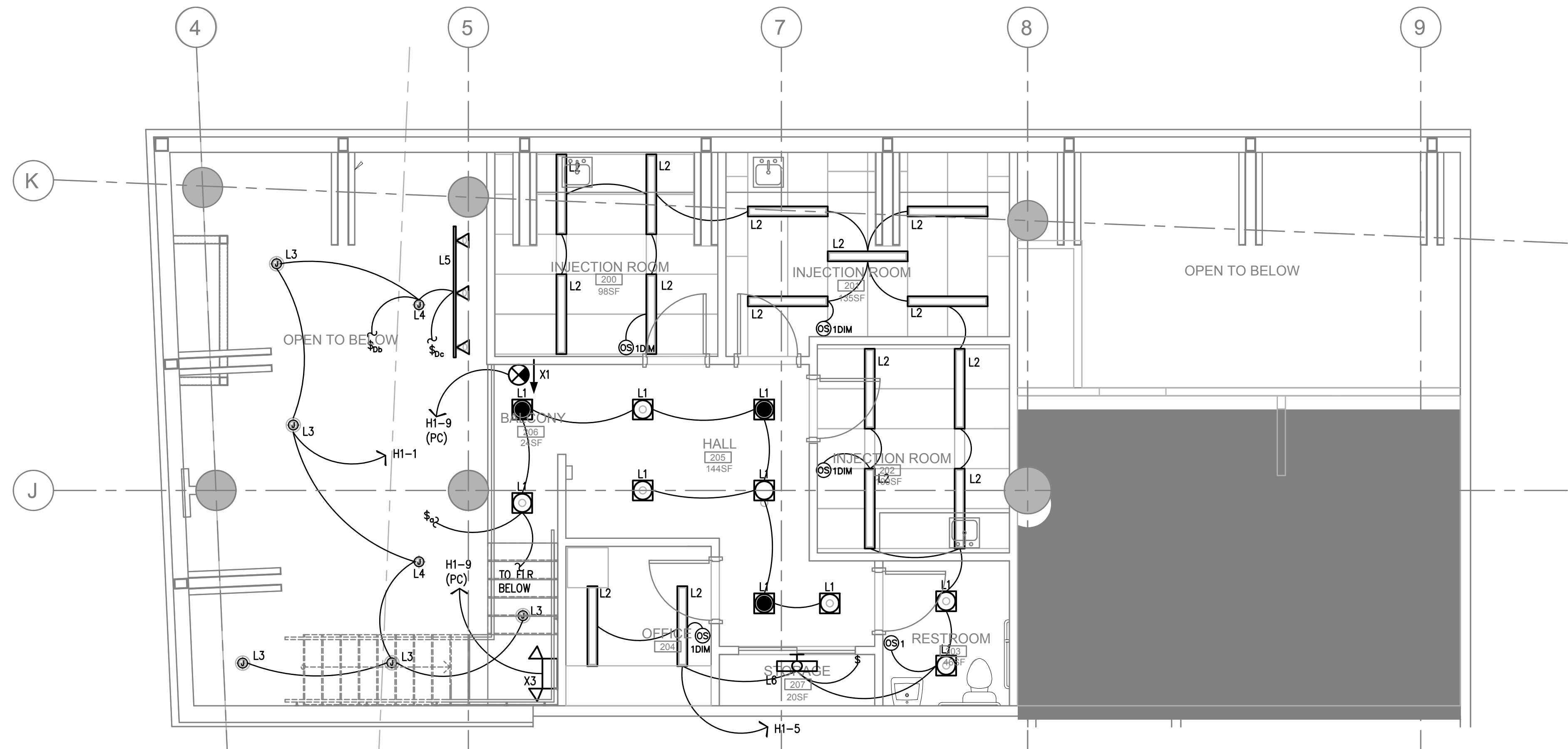
2 LIGHTING PLAN – MEZZANINE LEVEL E2.01 SCALE: 1/4" = 1'-0"
