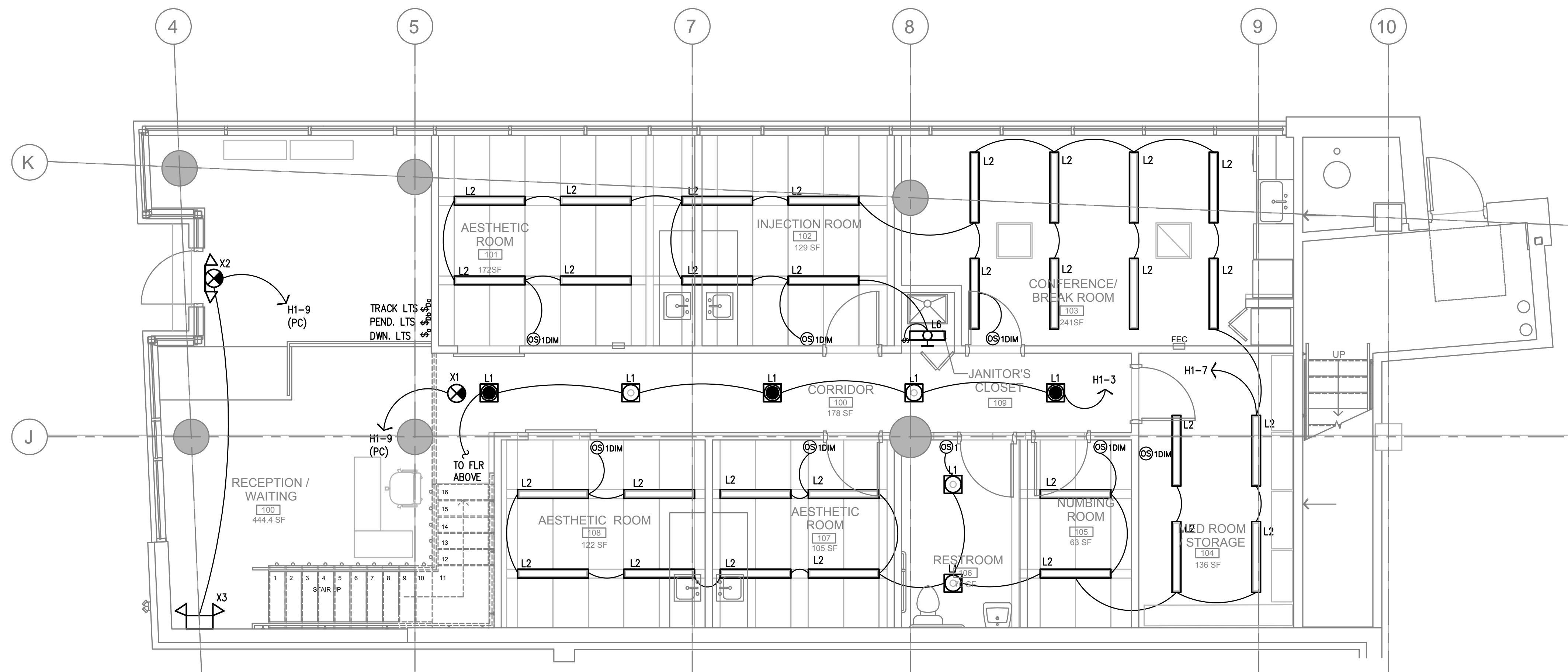
1 LIGHTING PLAN – MAIN LEVEL E2.01 SCALE: 1/4" = 1'-0"
