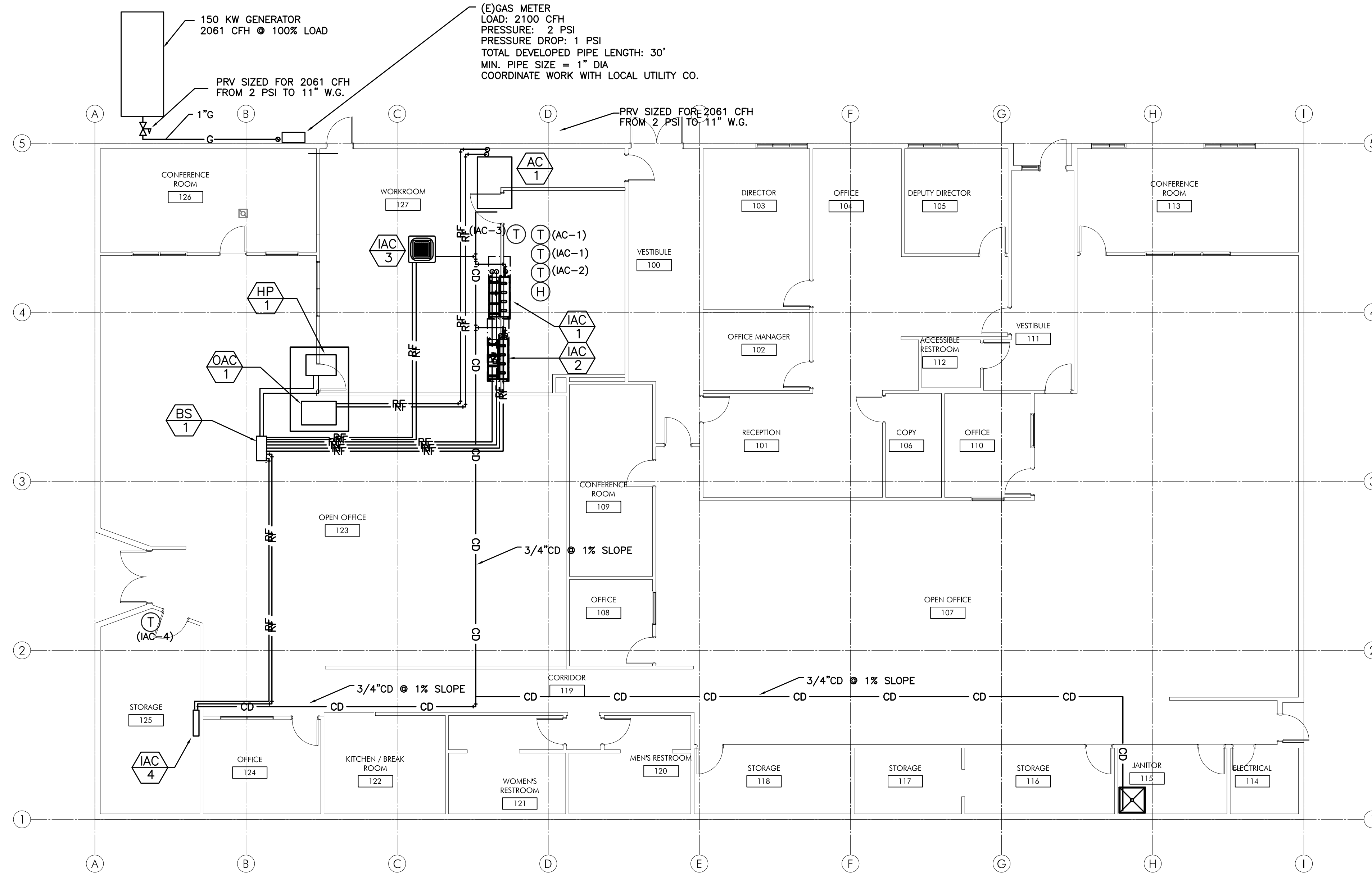
1 MECHANICAL PIPING PLAN M2.1 SCALE: 1/8" = 1'-0"
