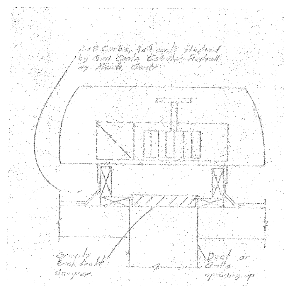
TYPICAL REF. INSTALLATION DETAIL (3) M-1 NO SCALE
