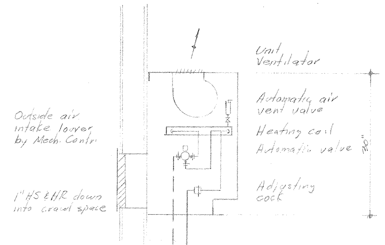
UNIT VENTILATOR INSTALLATION DETAIL (1) M-1 No Scale
