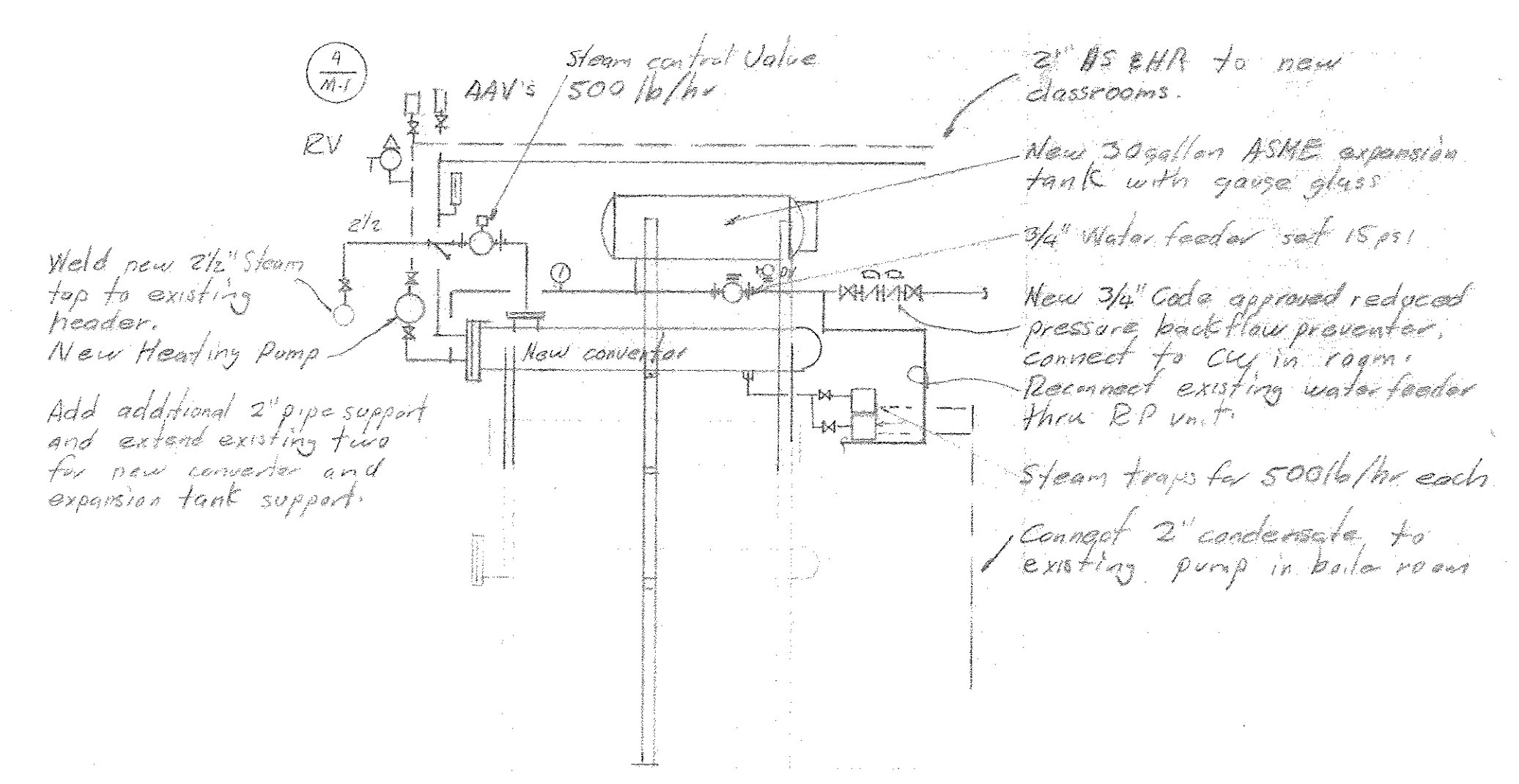
BOILER ROOM PIPING DIAGRAM (2) M-1 No Scale
