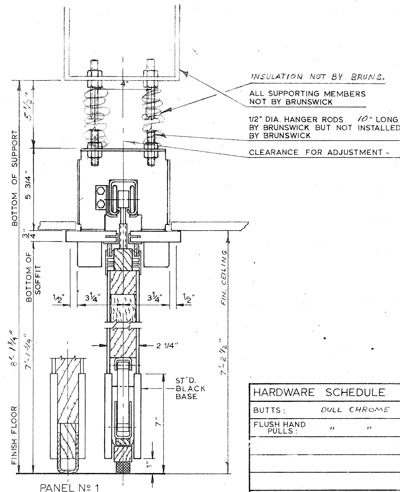
VERTICAL SECTION THRU PARTITION SCALE 3" = 1'-0"
