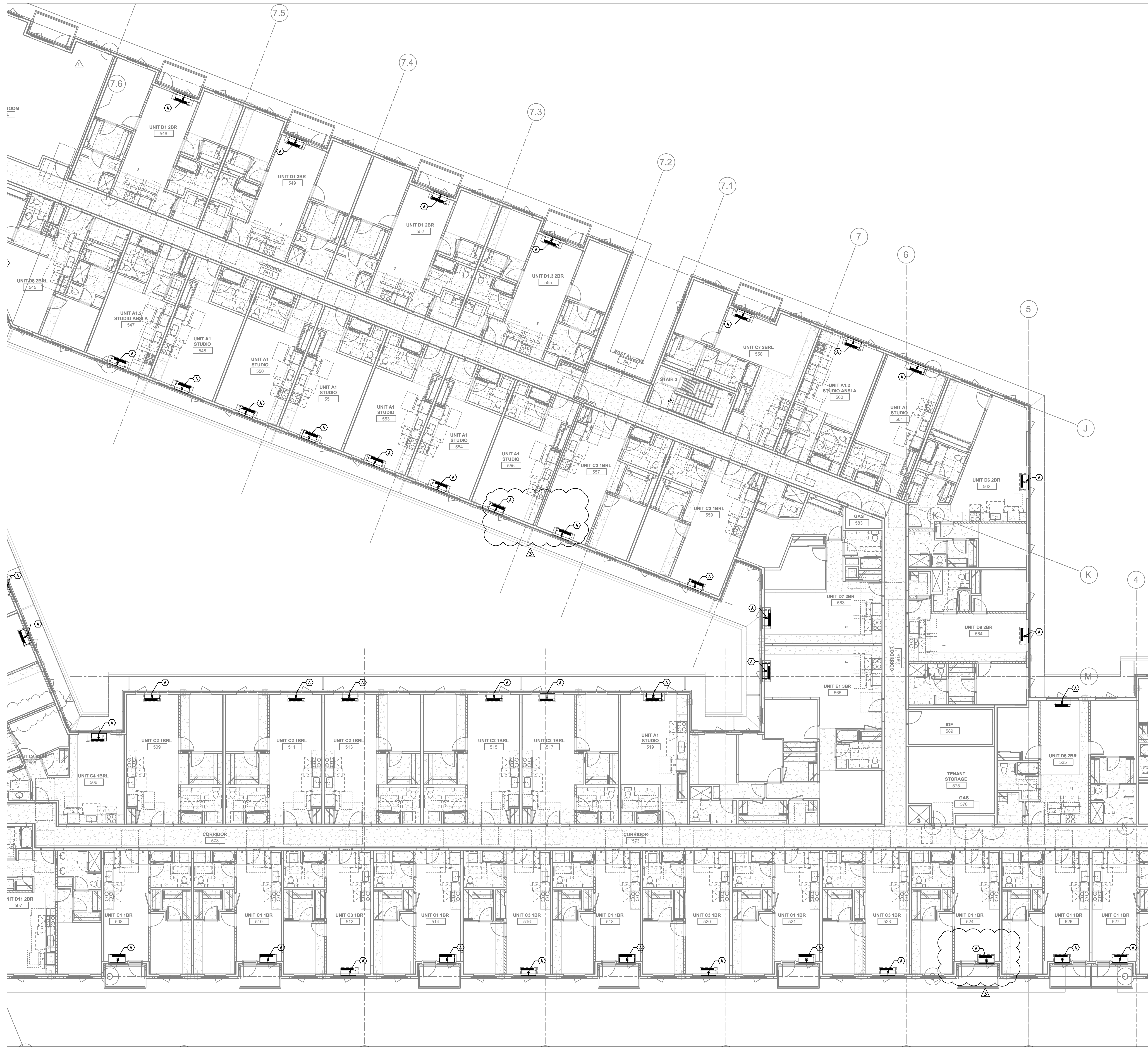
1 CONDENSATE FLOOR PLAN - LEVEL 05B M305B SCALE: 1/8" = 1'-0"
