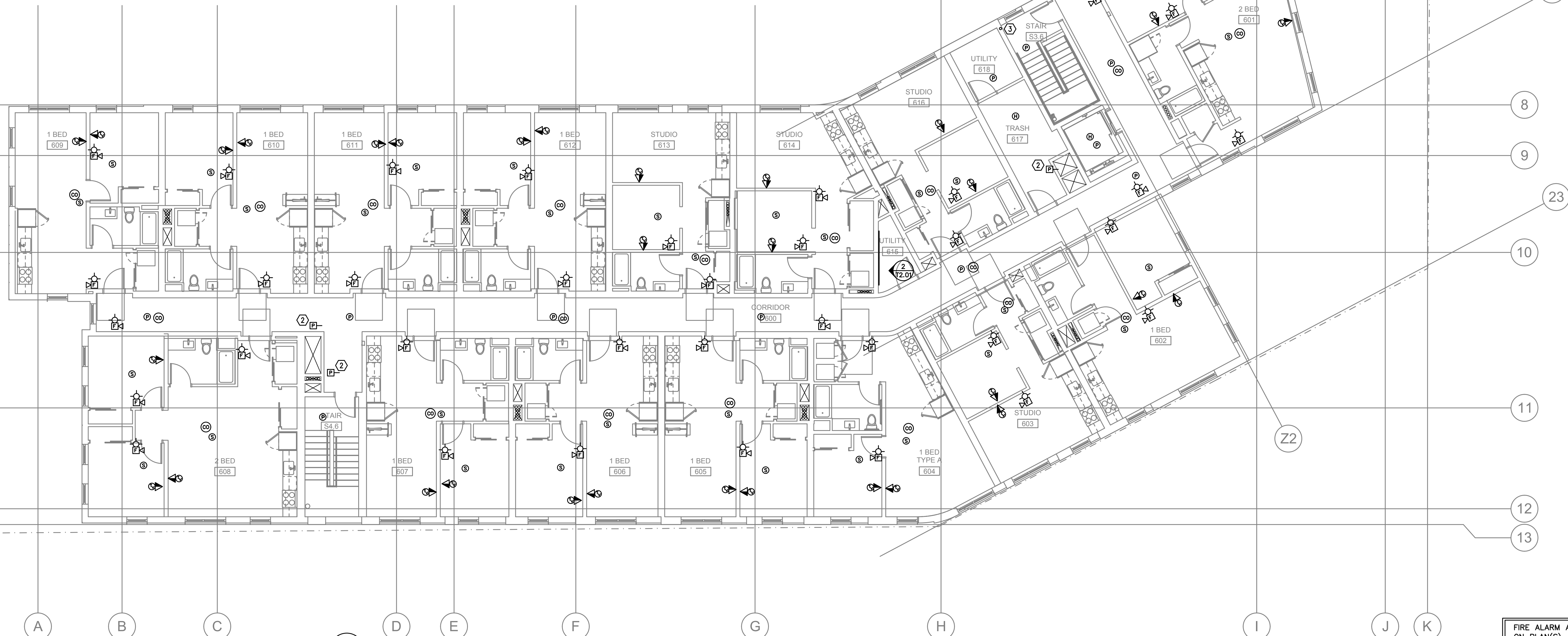
1 FLOOR PLAN - LEVEL 6 T3.06 1/8" = 1'-0"
