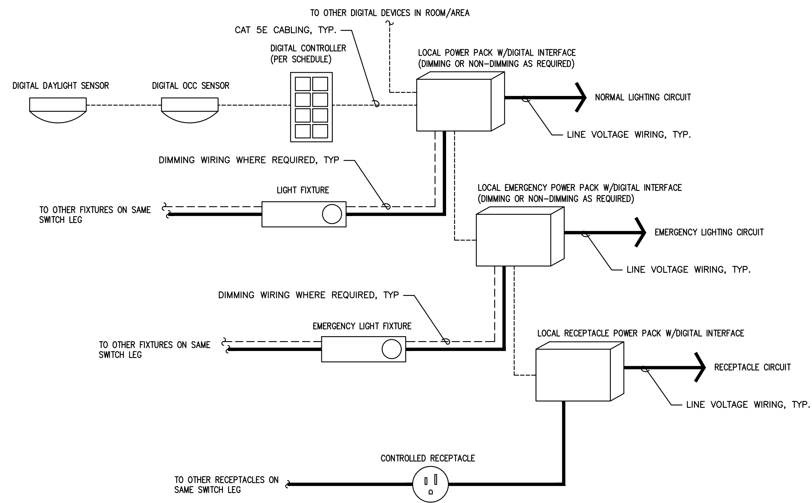
2 LIGHTING/RECEPTACLE CONTROL DIAGRAM E5.04 NTS
