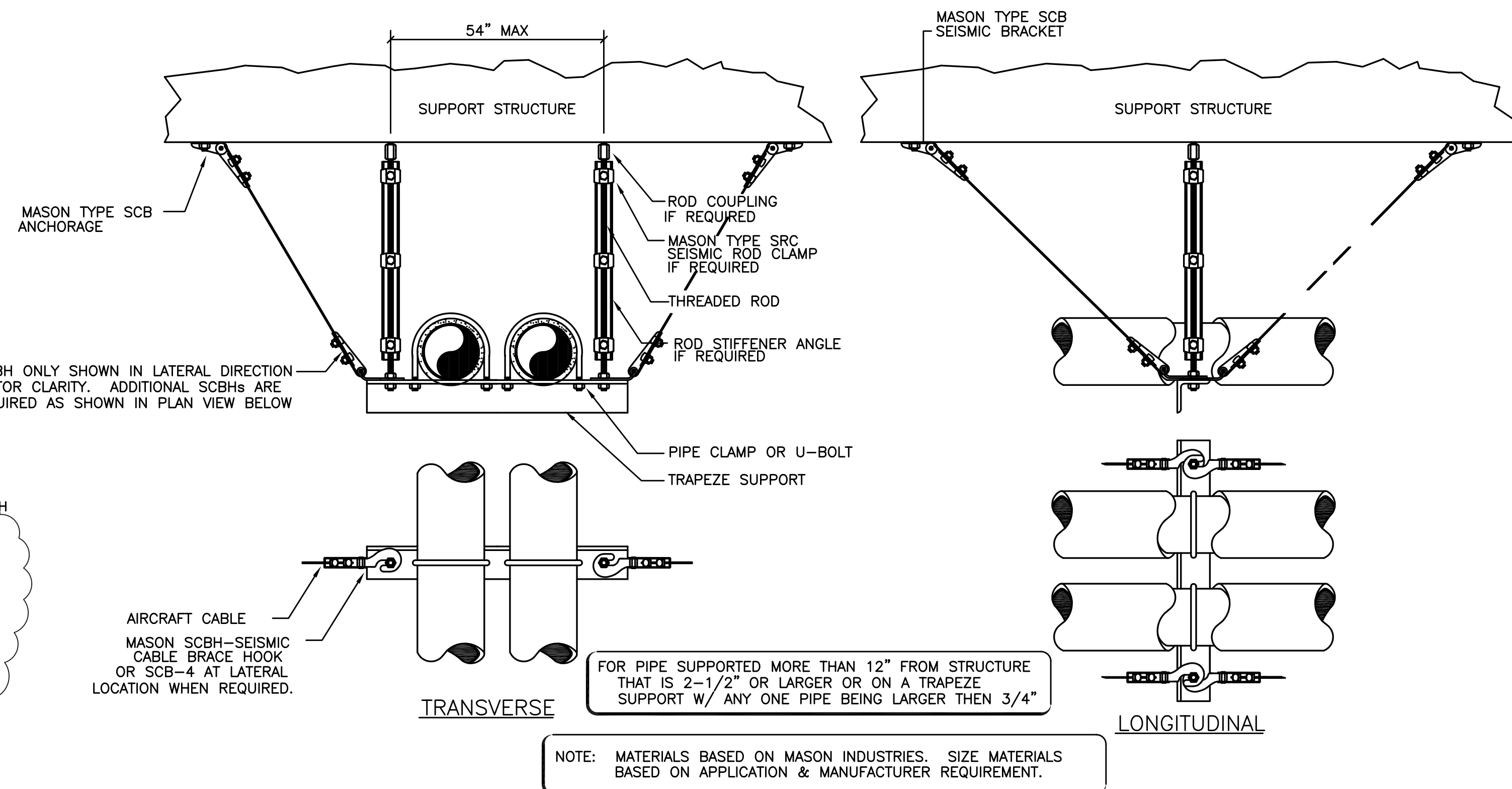
6 SEISMIC PIPE SUPPORT P6.01 SCALE: DETAIL
