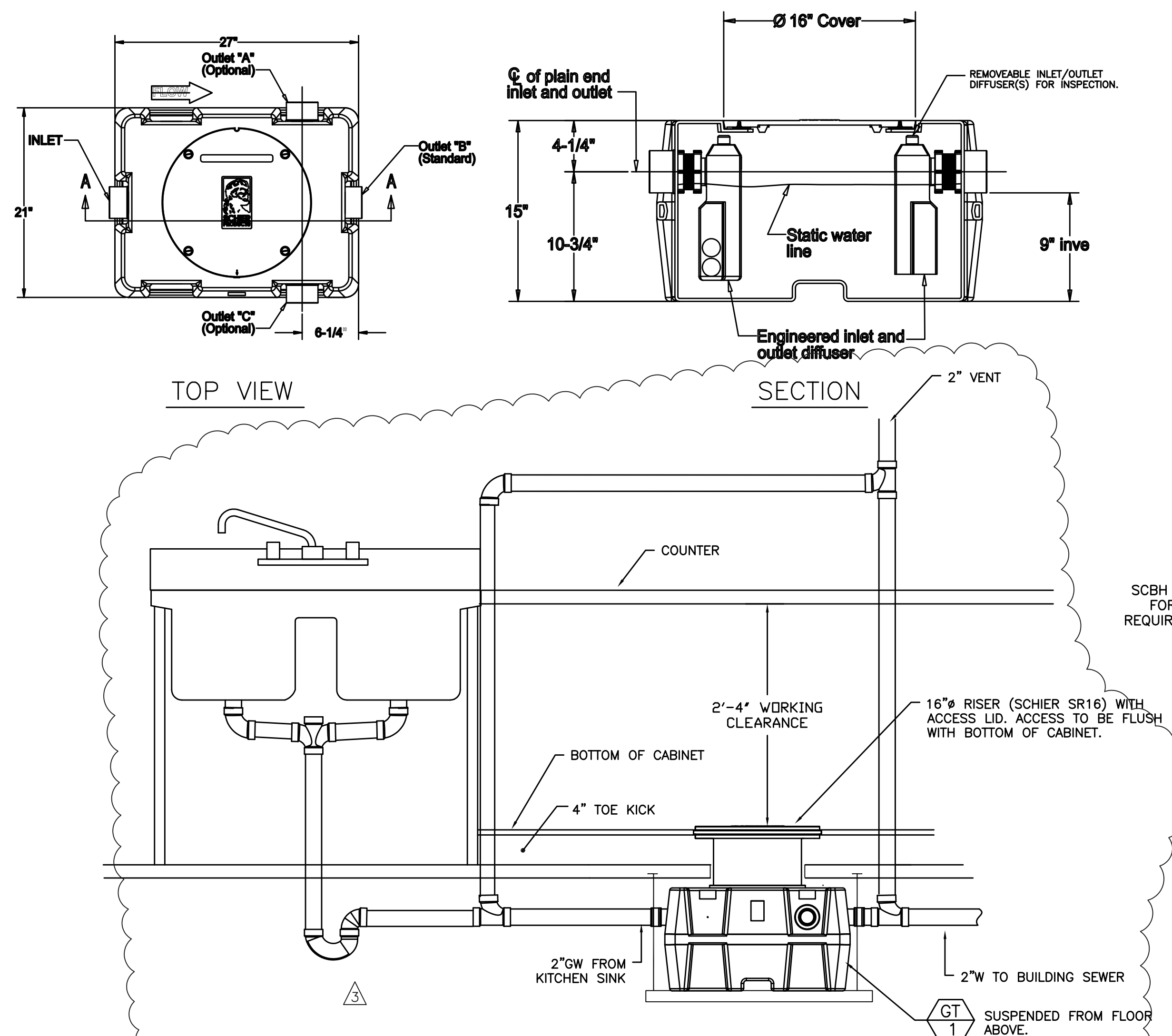
3 GREASE INTERCEPTOR DETAIL P6.01 SCALE: DETAIL
