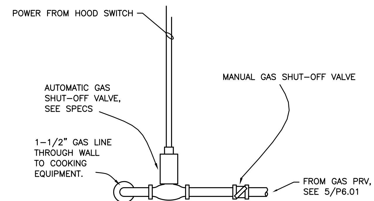
4 AUTO GAS SHUT-OFF ASSEMBLY P6.01 SCALE: NONE
