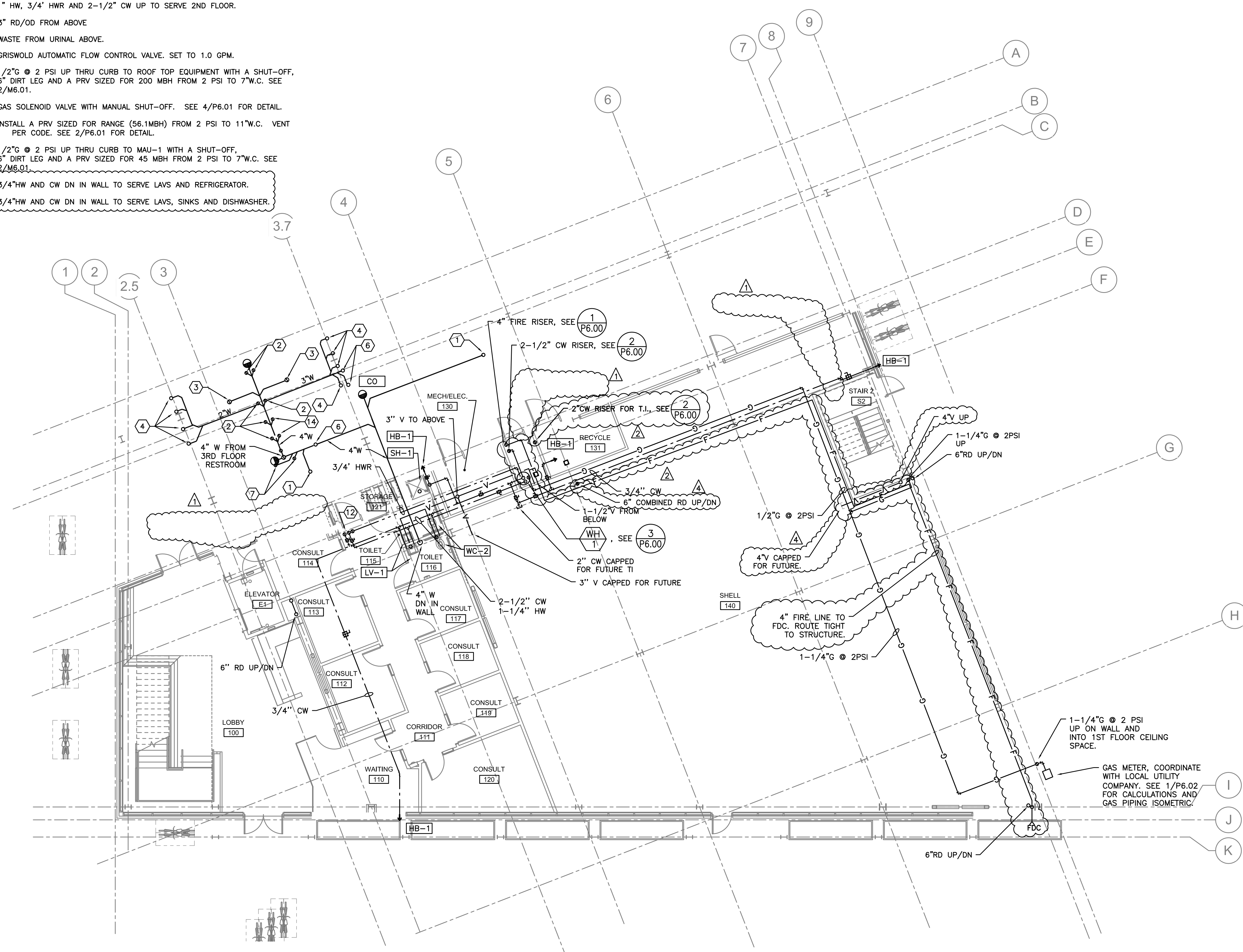
PROJECT NORTH 1 FIRST FLOOR PLUMBING PLAN SCALE: 1/8" = 1'-0"
