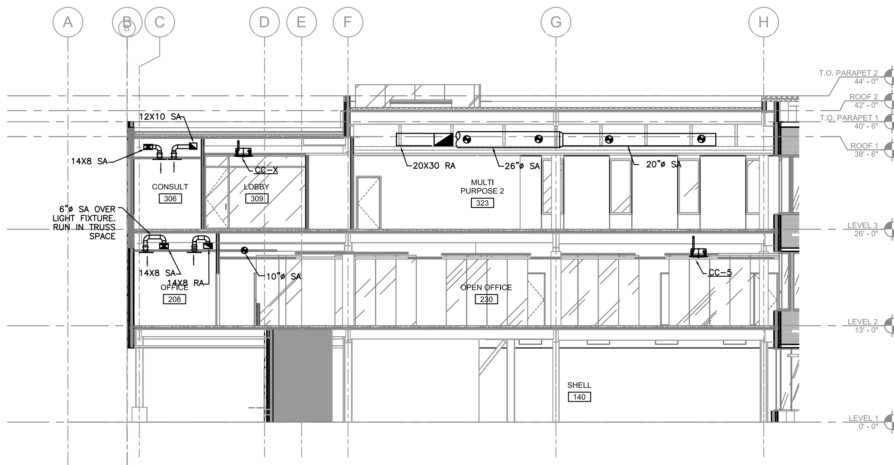
SECTION C
