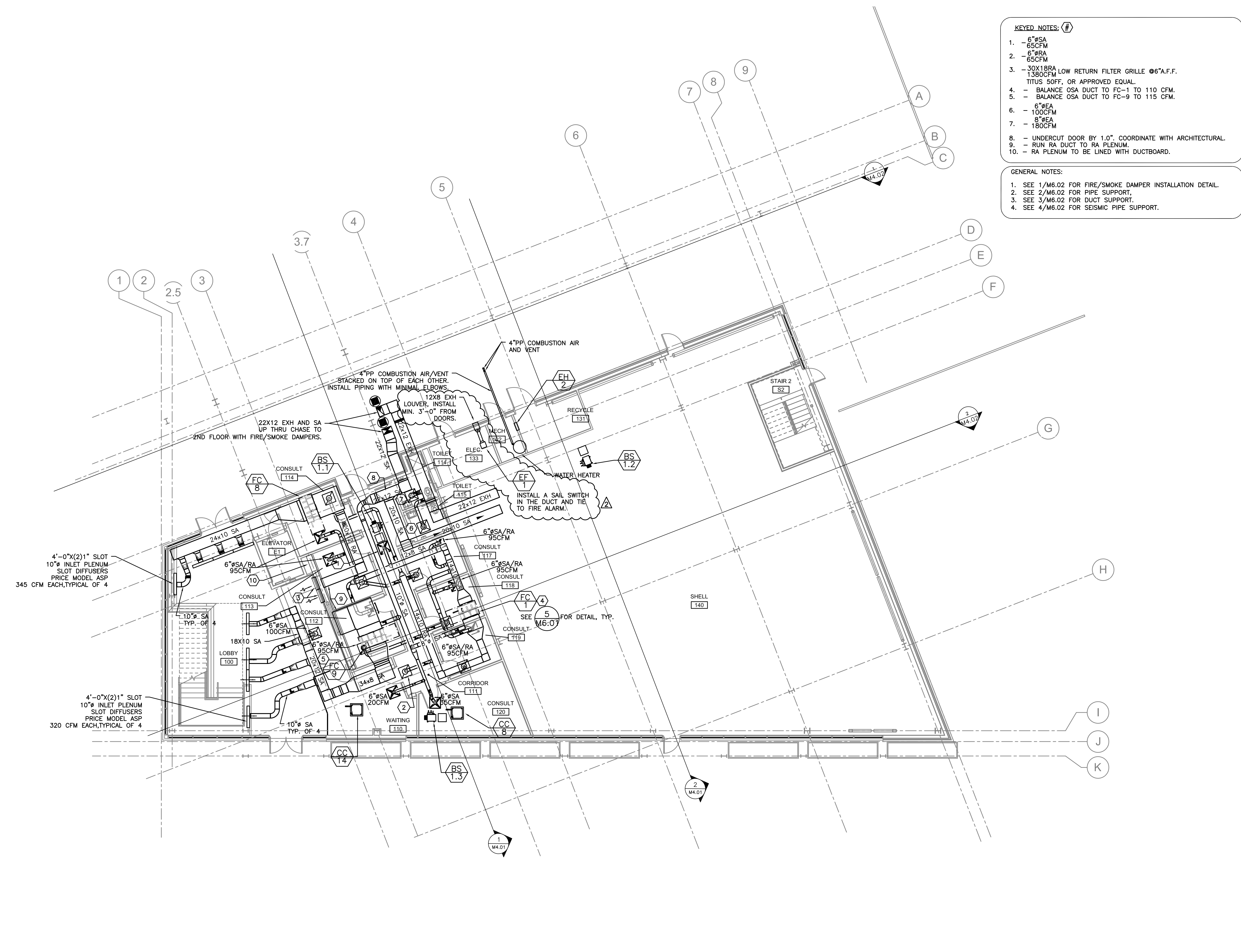
PROJECT NORTH 1 FIRST FLOOR MECHANICAL PLAN SCALE: 1/8" = 1'-0" M2.01
