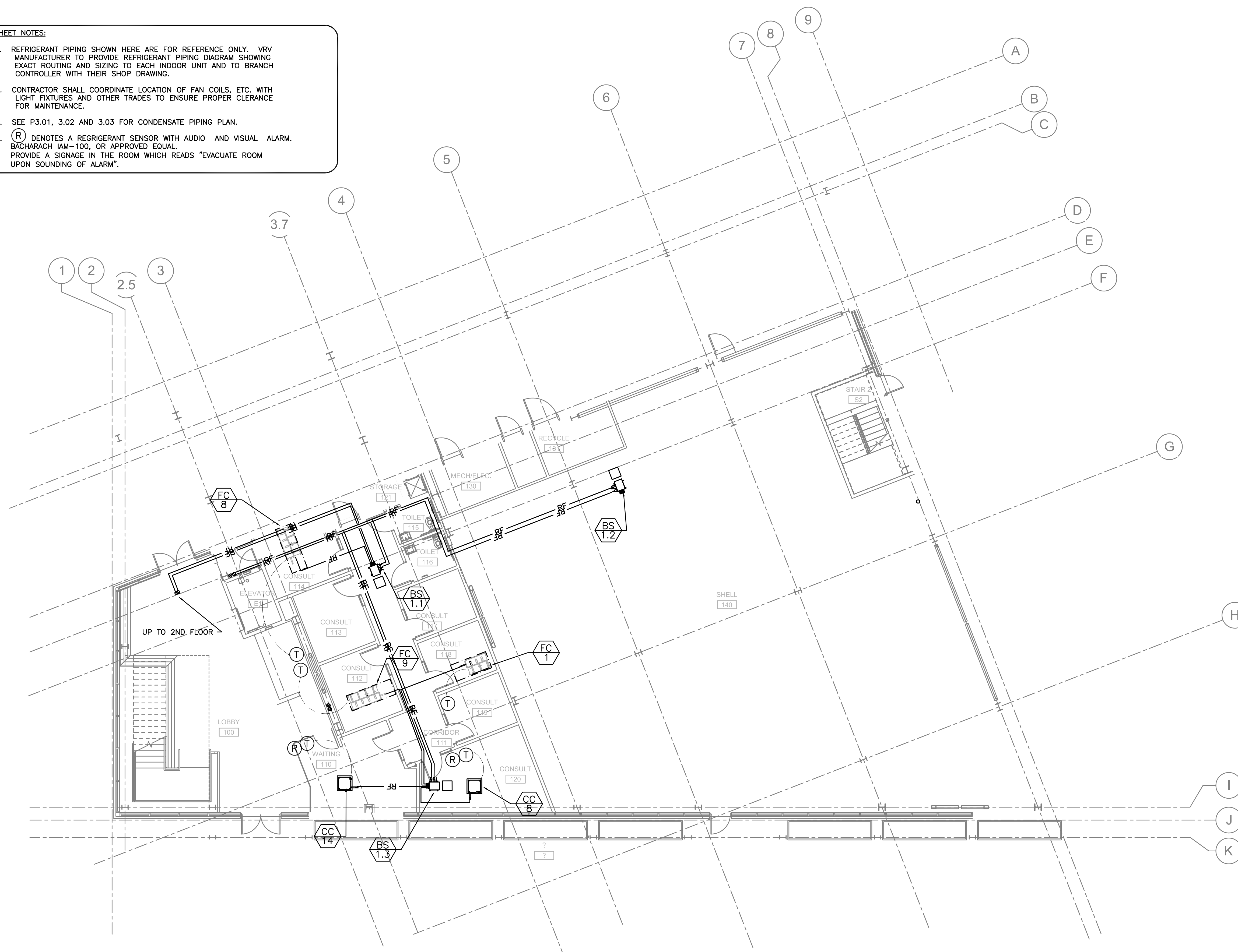
1 FIRST FLOOR REFRIGERANT PIPING PLAN SCALE: 1/8" = 1'-0"
