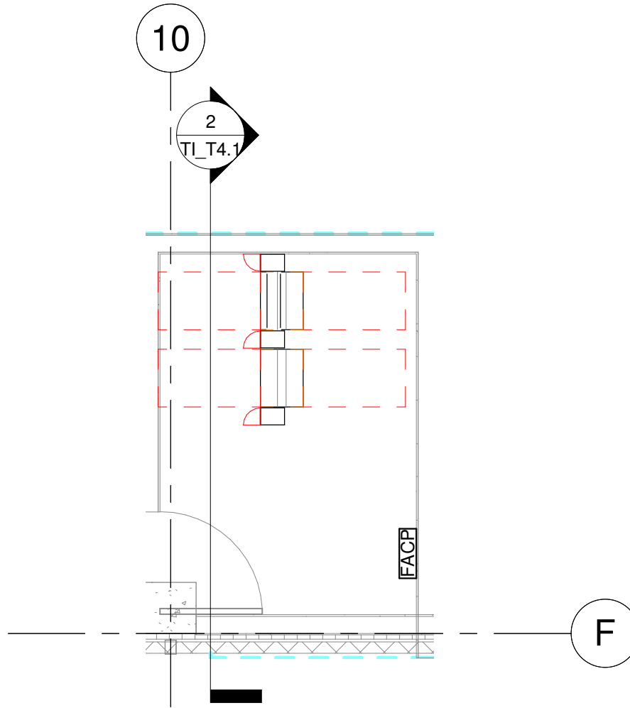
1 ENLARGED SERVER 163 1/4" = 1'-0"
