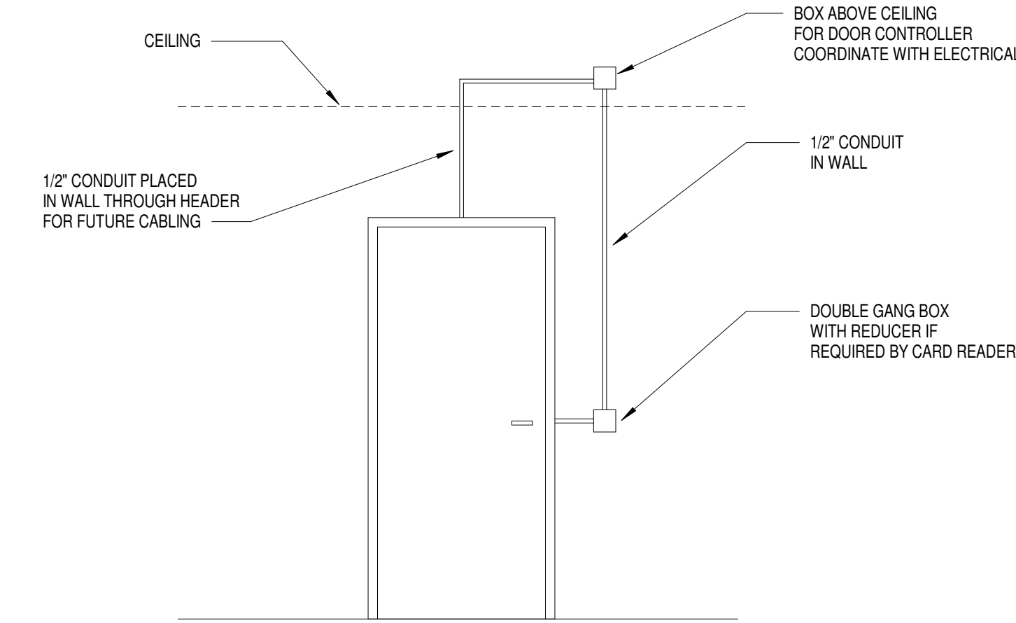
3 ACCESS CONTROL ROUGH-IN DETAIL 1/2" = 1'-0"
