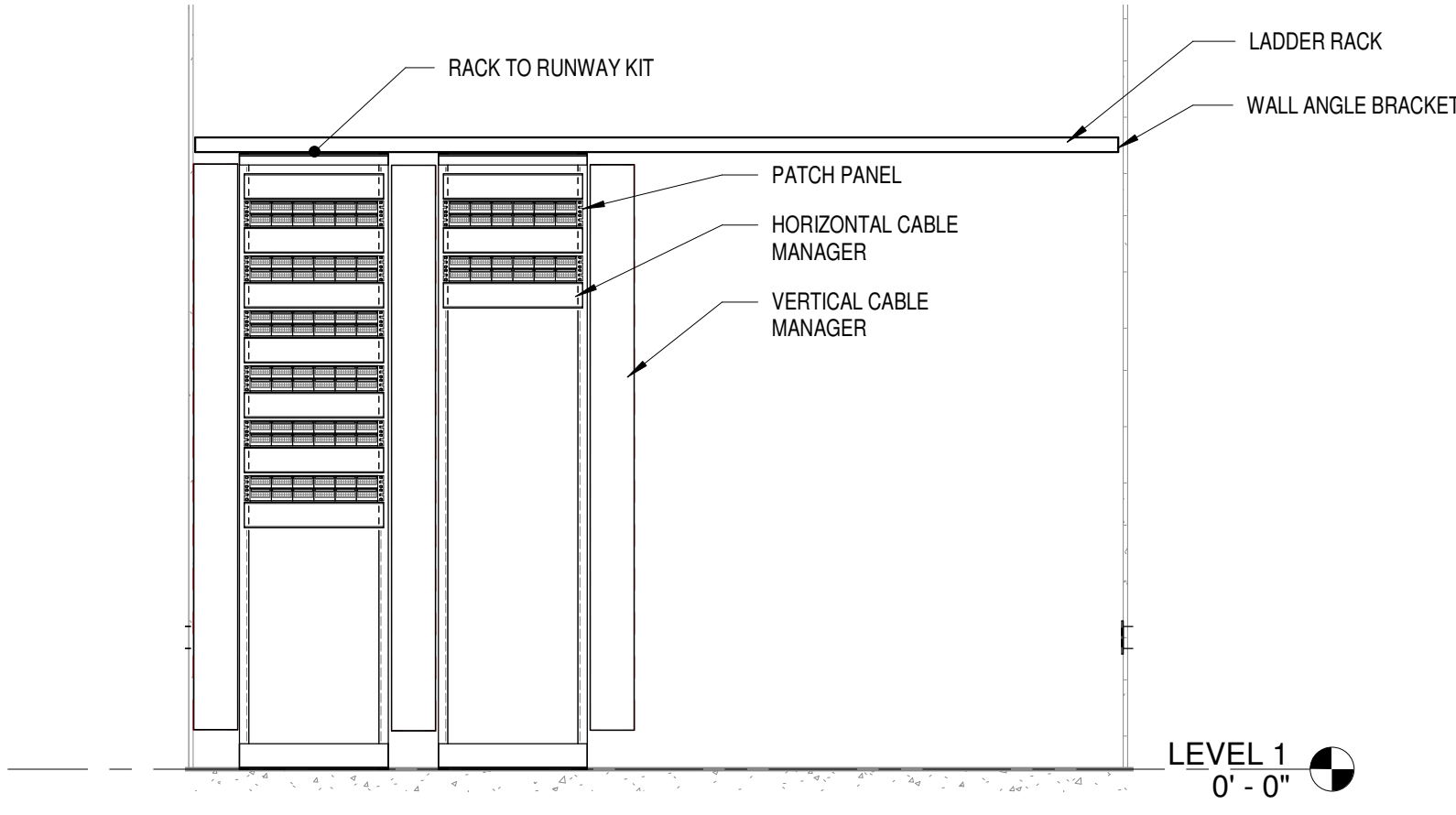
2 DATA RACK ELEVATIONS 1/2" = 1'-0"
