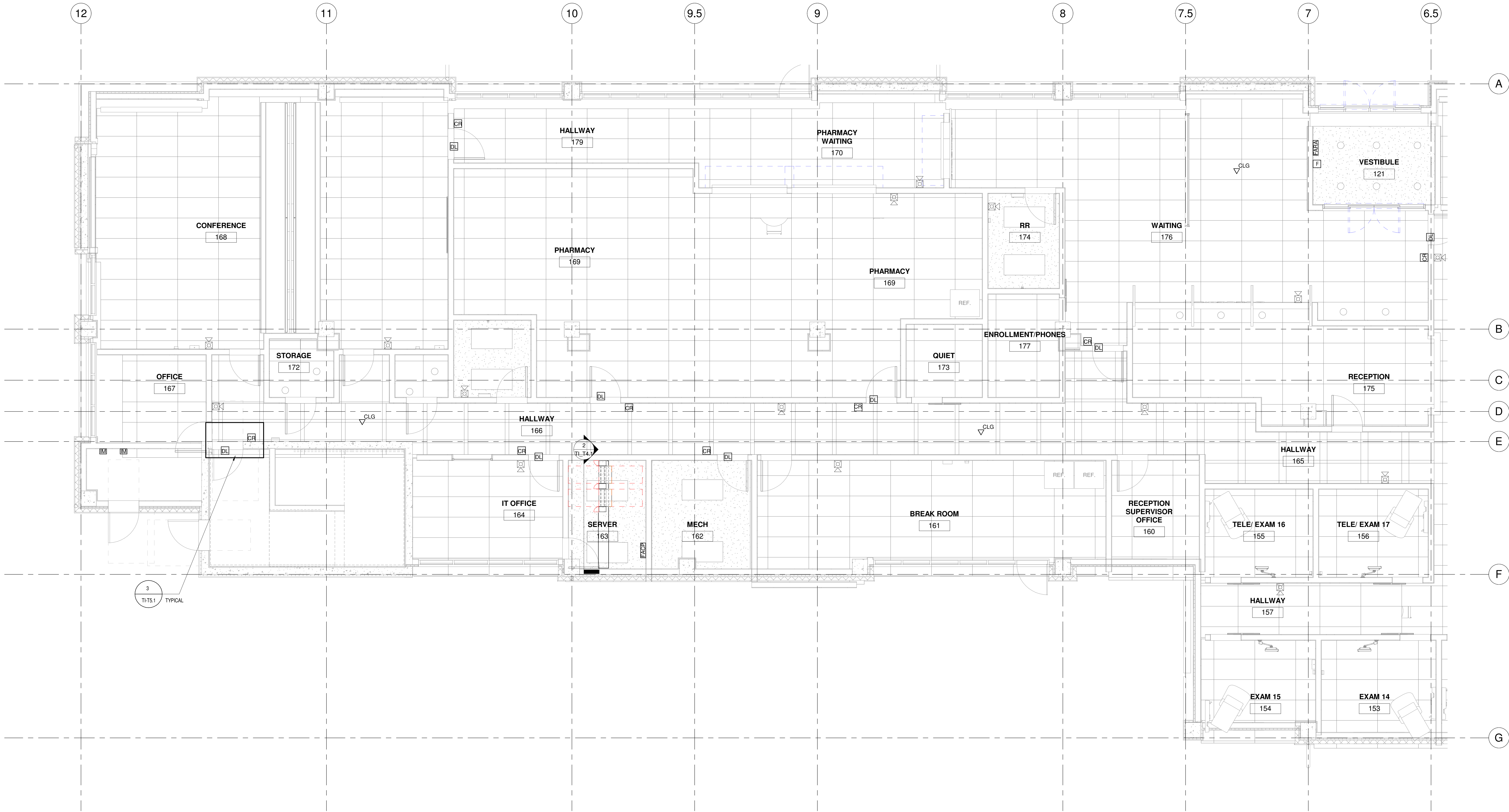
1 FIRST FLOOR SOUTH - TECHNOLOGY CEILING 1/4" = 1'-0"
