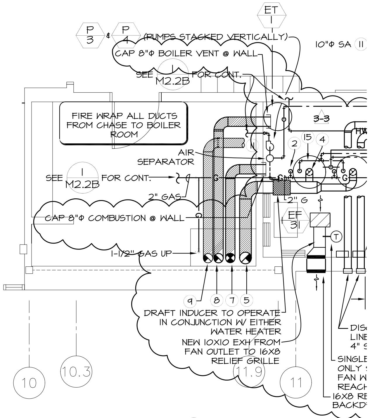
1 M6.2 BOILER ROOM I 1/4"=1'-0"
