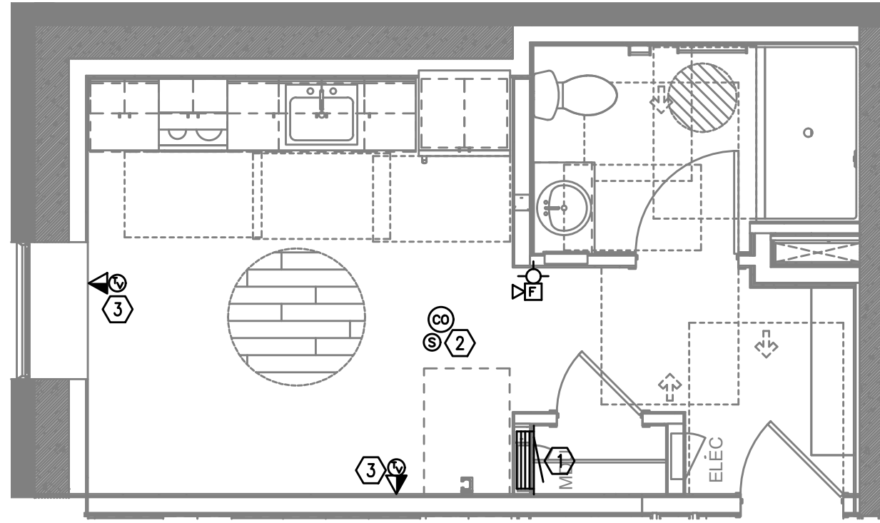
UNIT TYPE 11A TYPICAL TELCOM PLAN 2 T4.06 SCALE: 1/4" = 1'-0"
