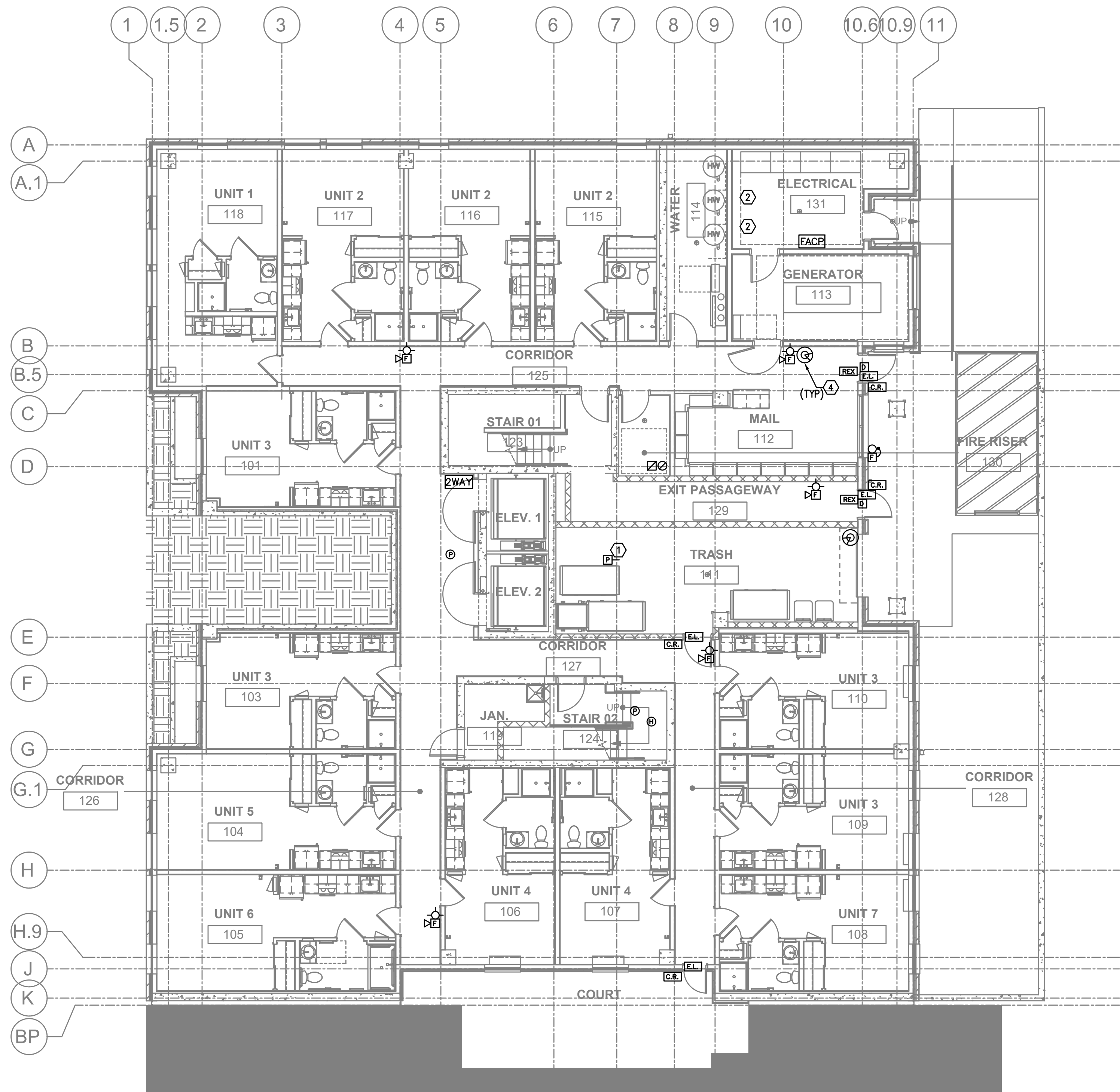
1 FIRST FLOOR TECHNOLOGY PLAN T3.01 SCALE: 1/8" = 1'-0"
