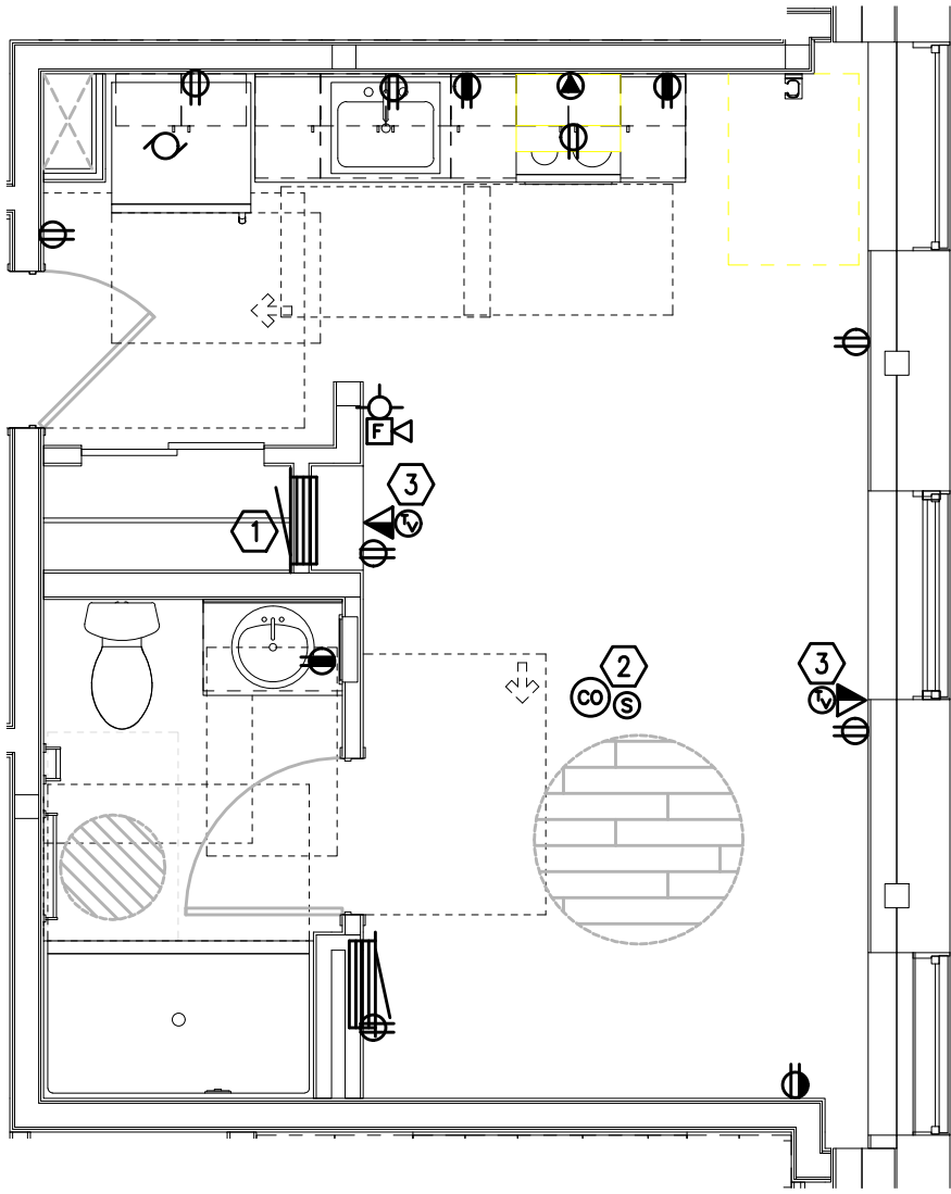
2 T4.04 UNIT TYPE 8A TYPICAL TELCOM PLAN SCALE: 1/4" = 1'-0"
