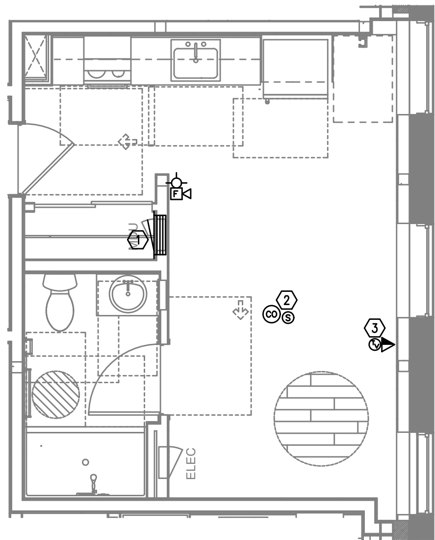
UNIT TYPE 8A TYPICAL TELCOM PLAN 2 T4.04 SCALE: 1/4" = 1'-0"
