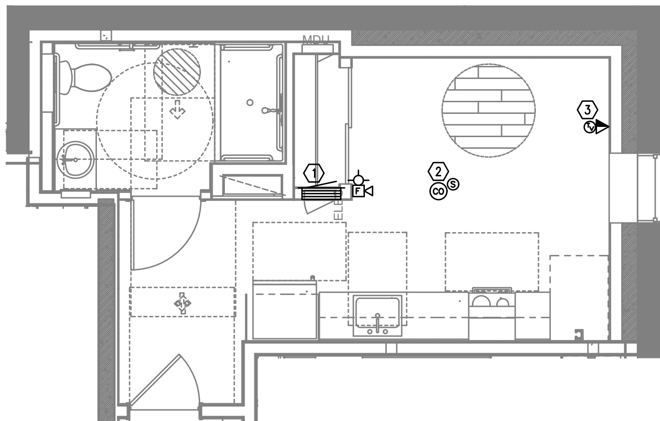
UNIT TYPE 9 TYPICAL TELCOM PLAN 3 T4.04 SCALE: 1/4" = 1'-0"
