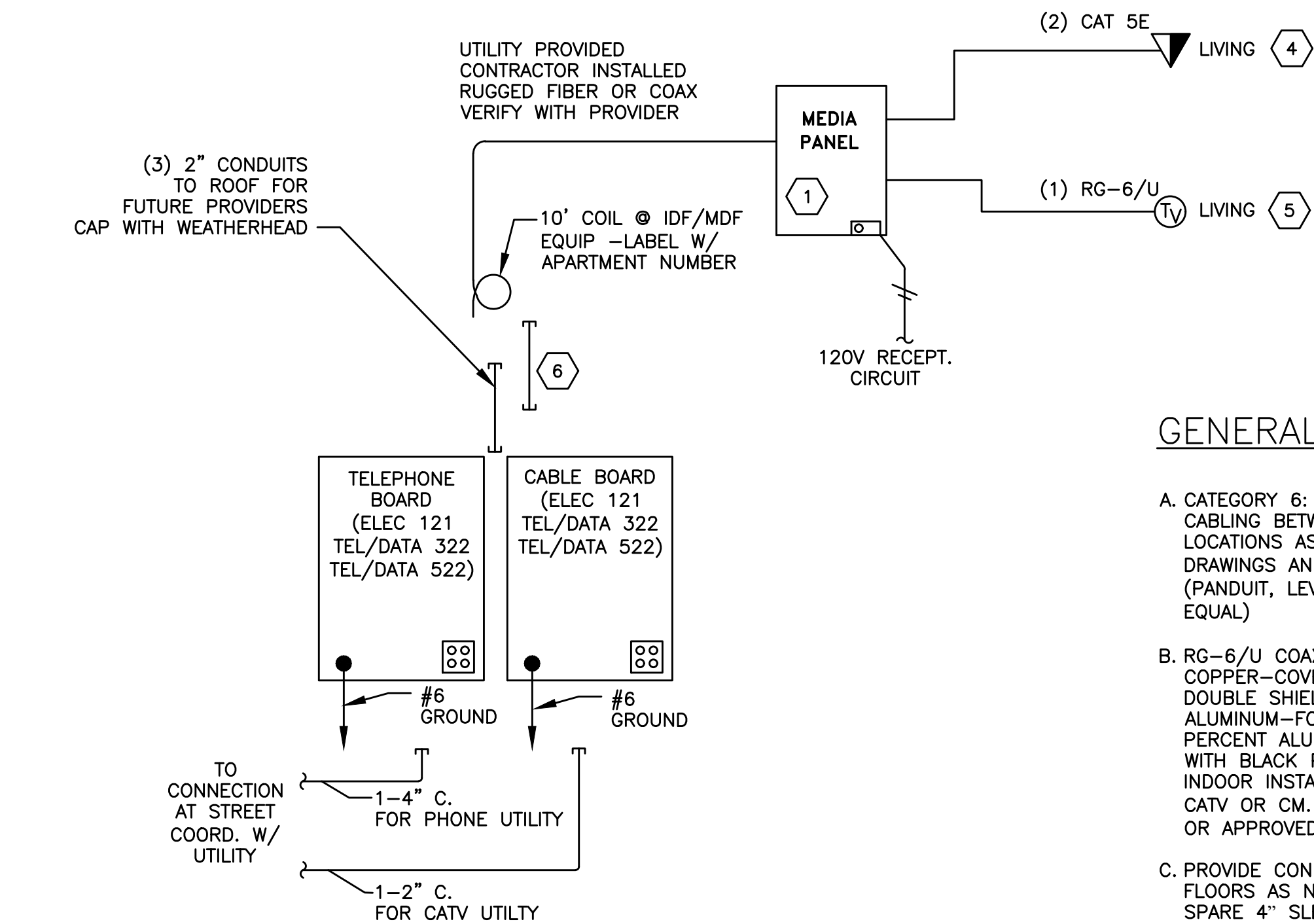
1 TELCOM CABLING DETAIL T2.02 N.T.S.
