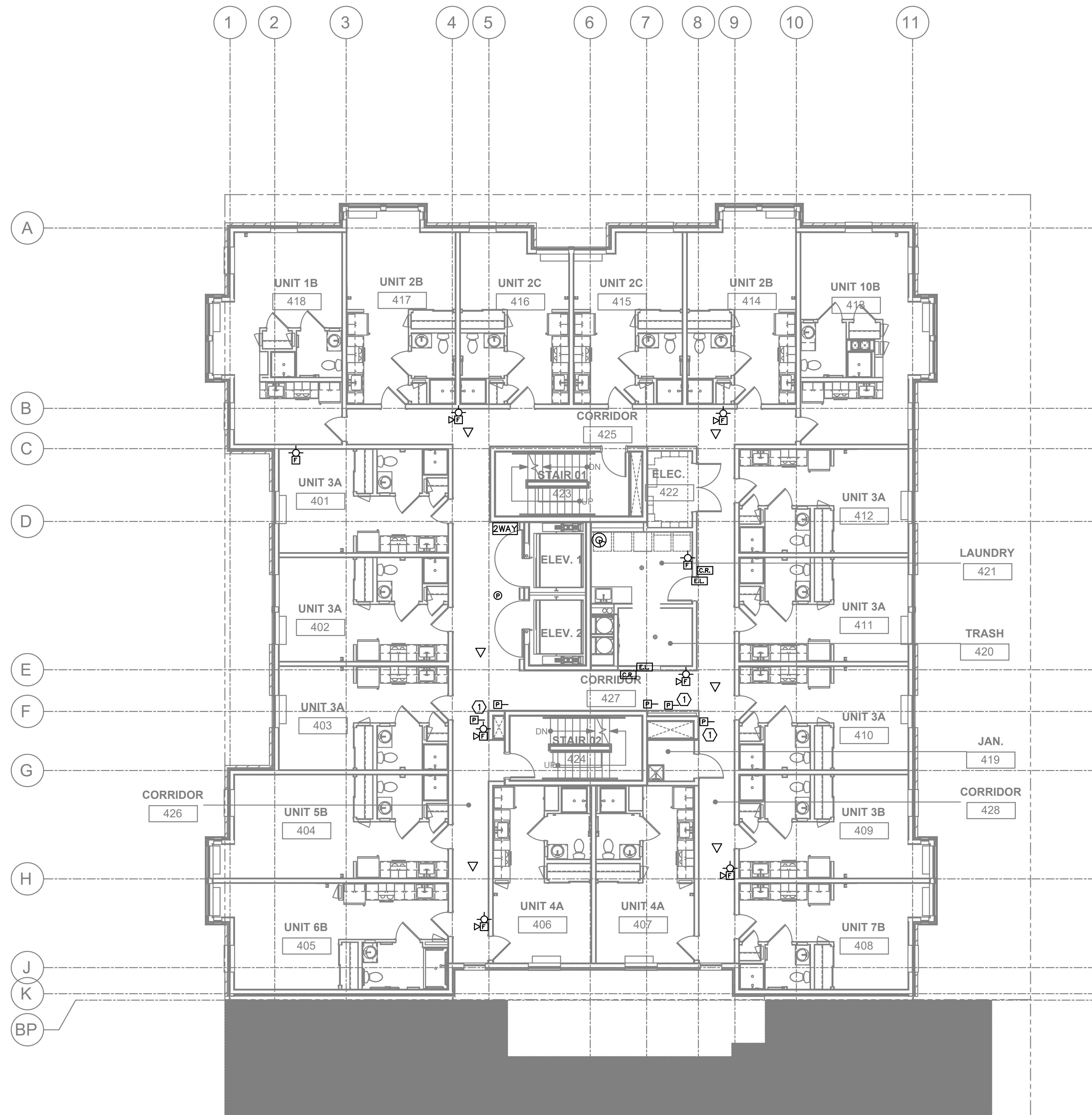
1 T3.04 FOURTH FLOOR TECHNOLOGY PLAN SCALE: 1/8" = 1'-0"
