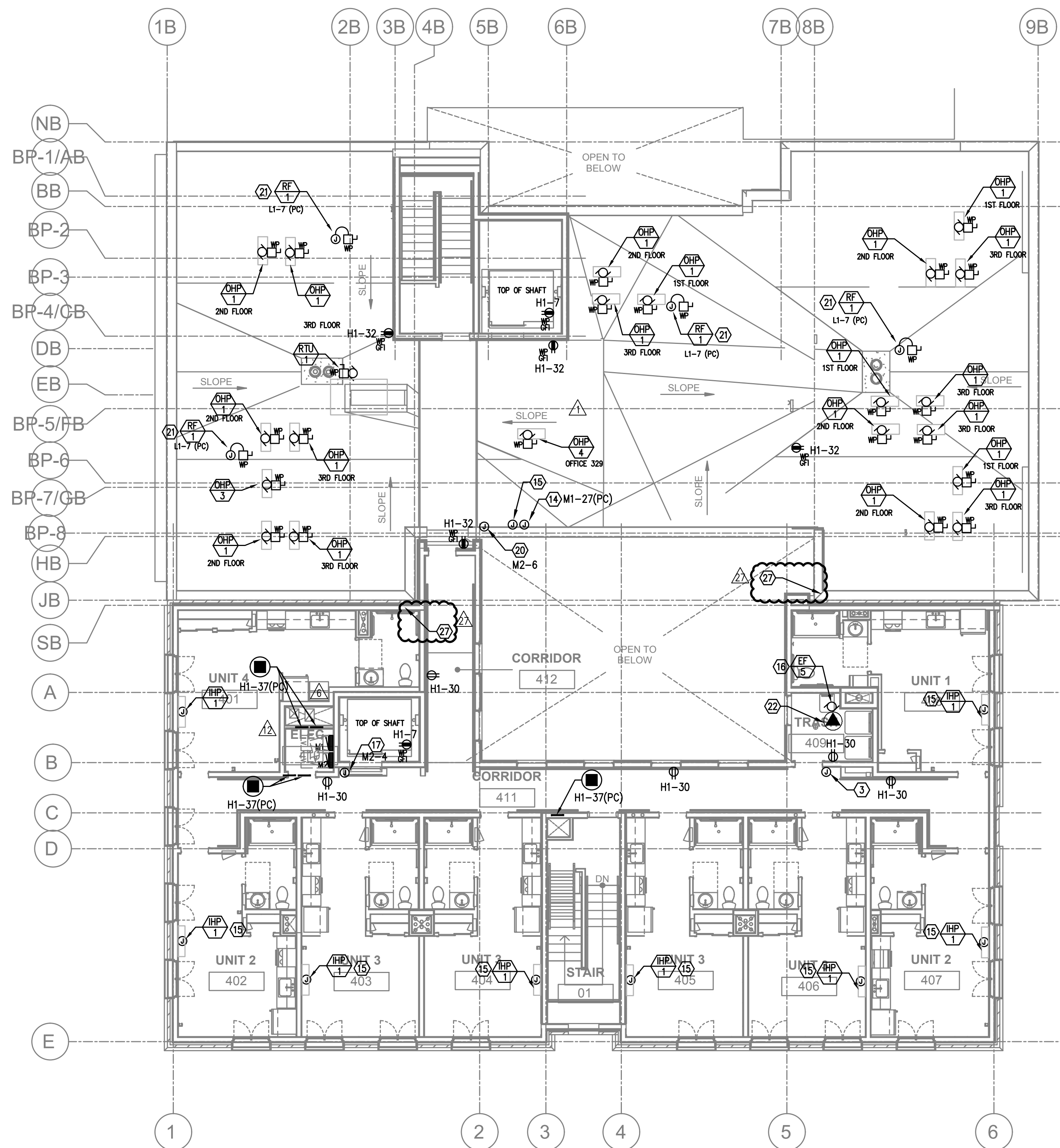
1 FOURTH FLOOR POWER PLAN E3.04 SCALE: 1/8" = 1'-0"
