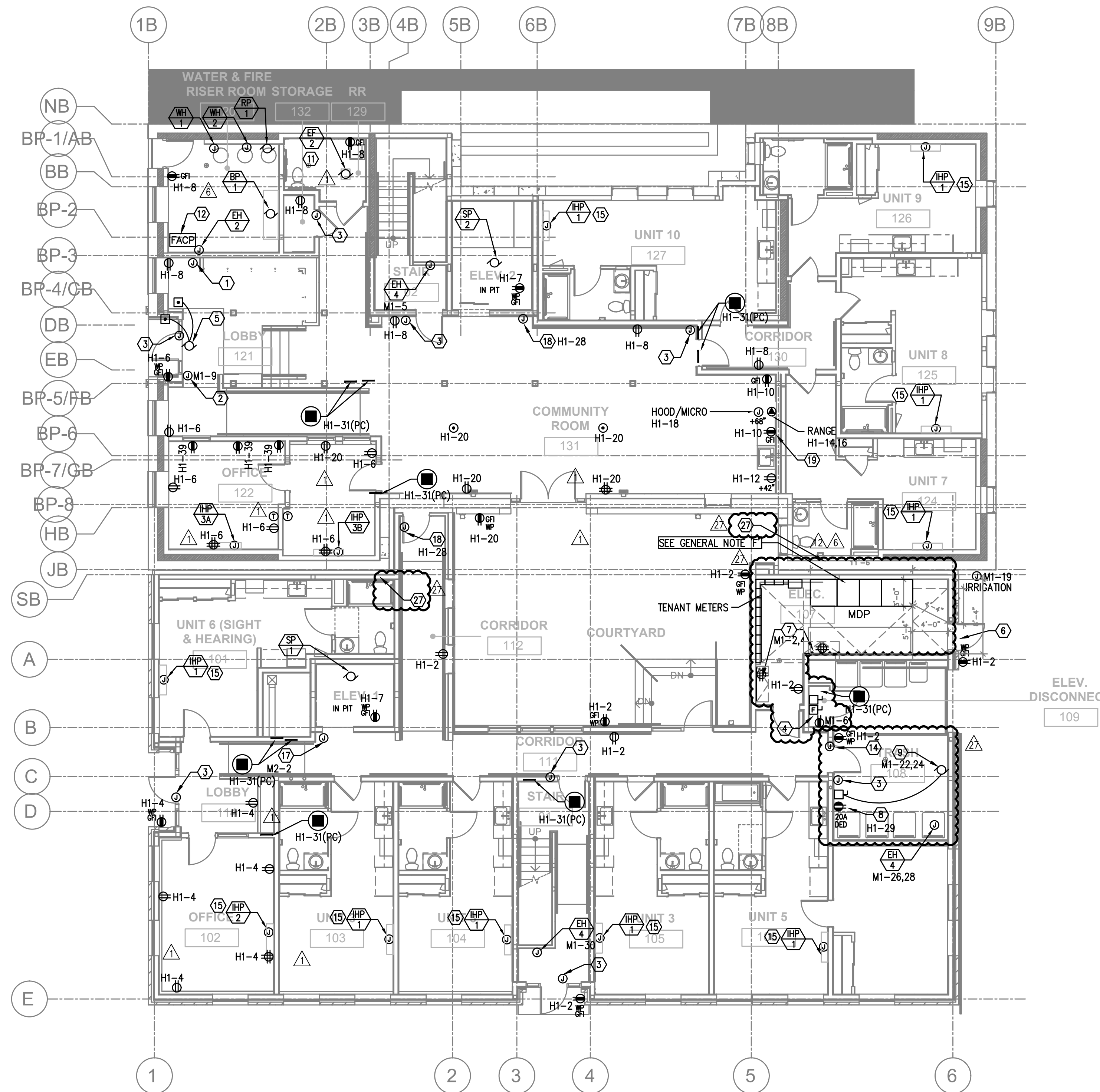
1 FIRST FLOOR POWER PLAN SCALE: 1/8" = 1'-0"
