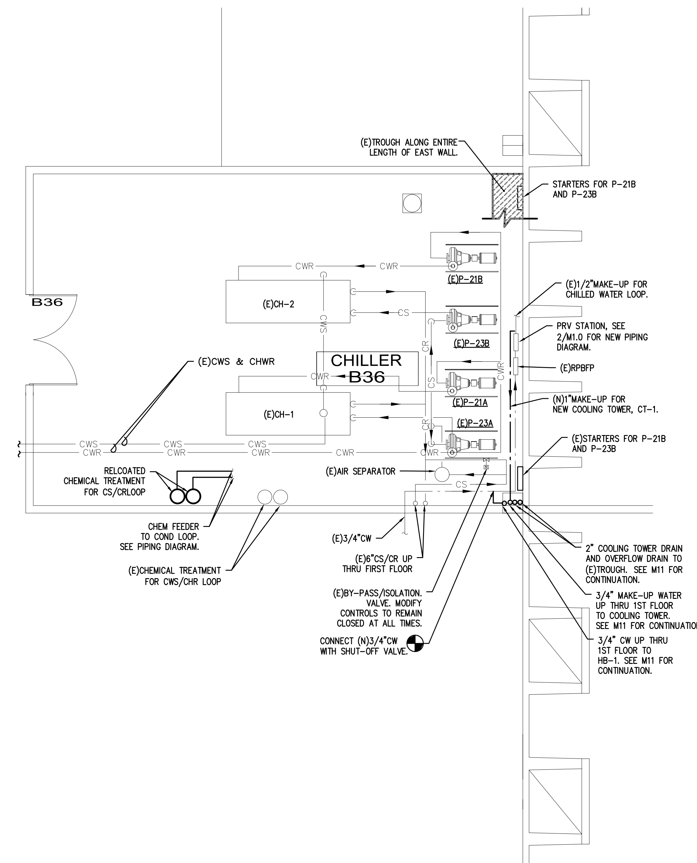
1 CHILLER ROOM - BASEMENT PIPING PLAN SCALE: 1/4" = 1'-0"
