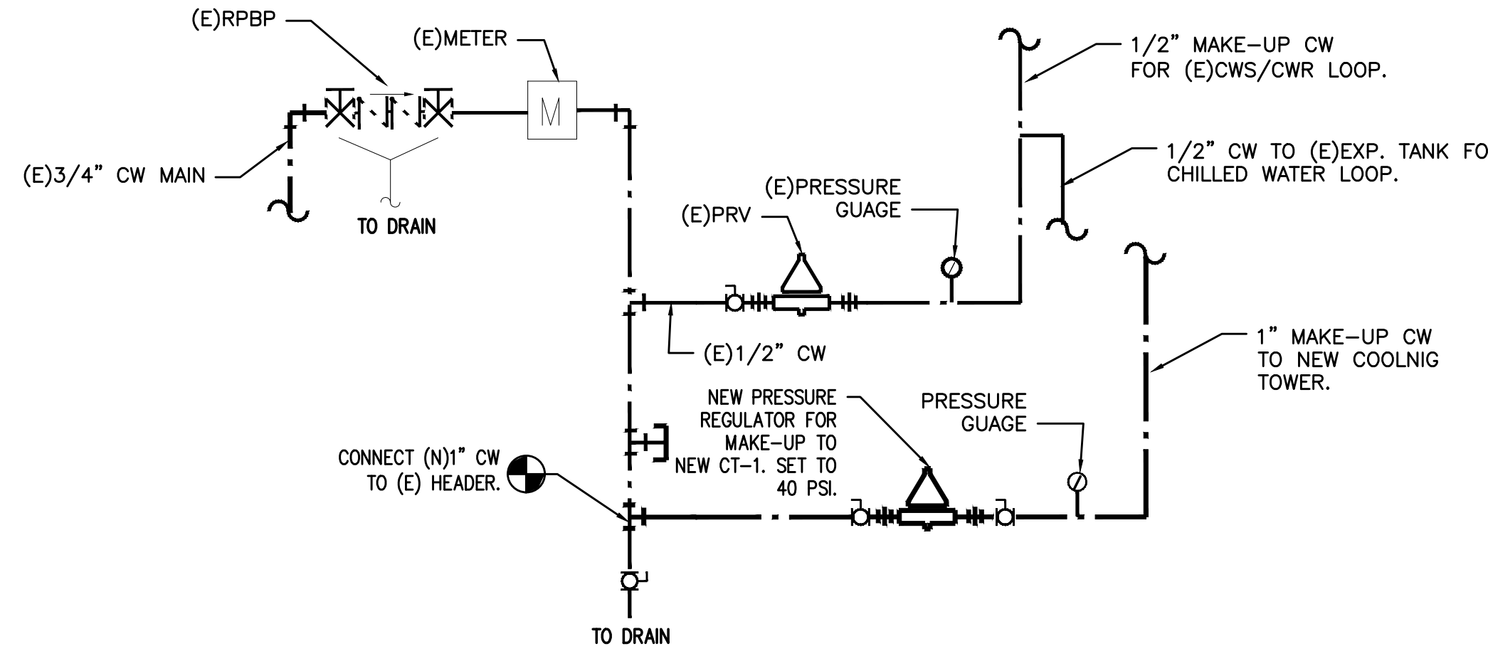
2 PRV STATION PIPING DETAIL M1.0 NO SCALE
