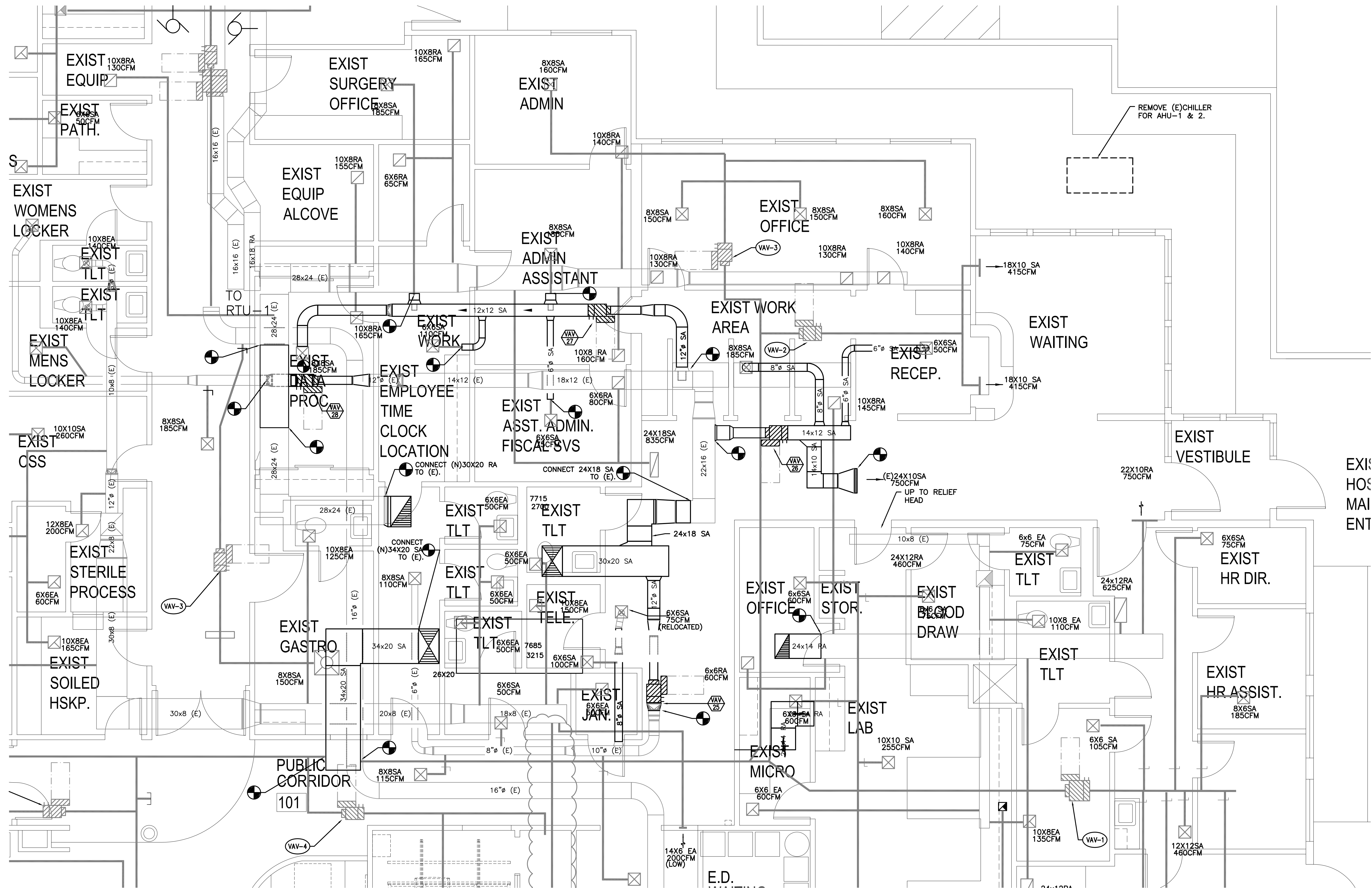
1 PARTIAL FLOOR PLAN M2.1 SCALE: 1/4" = 1'-0"
