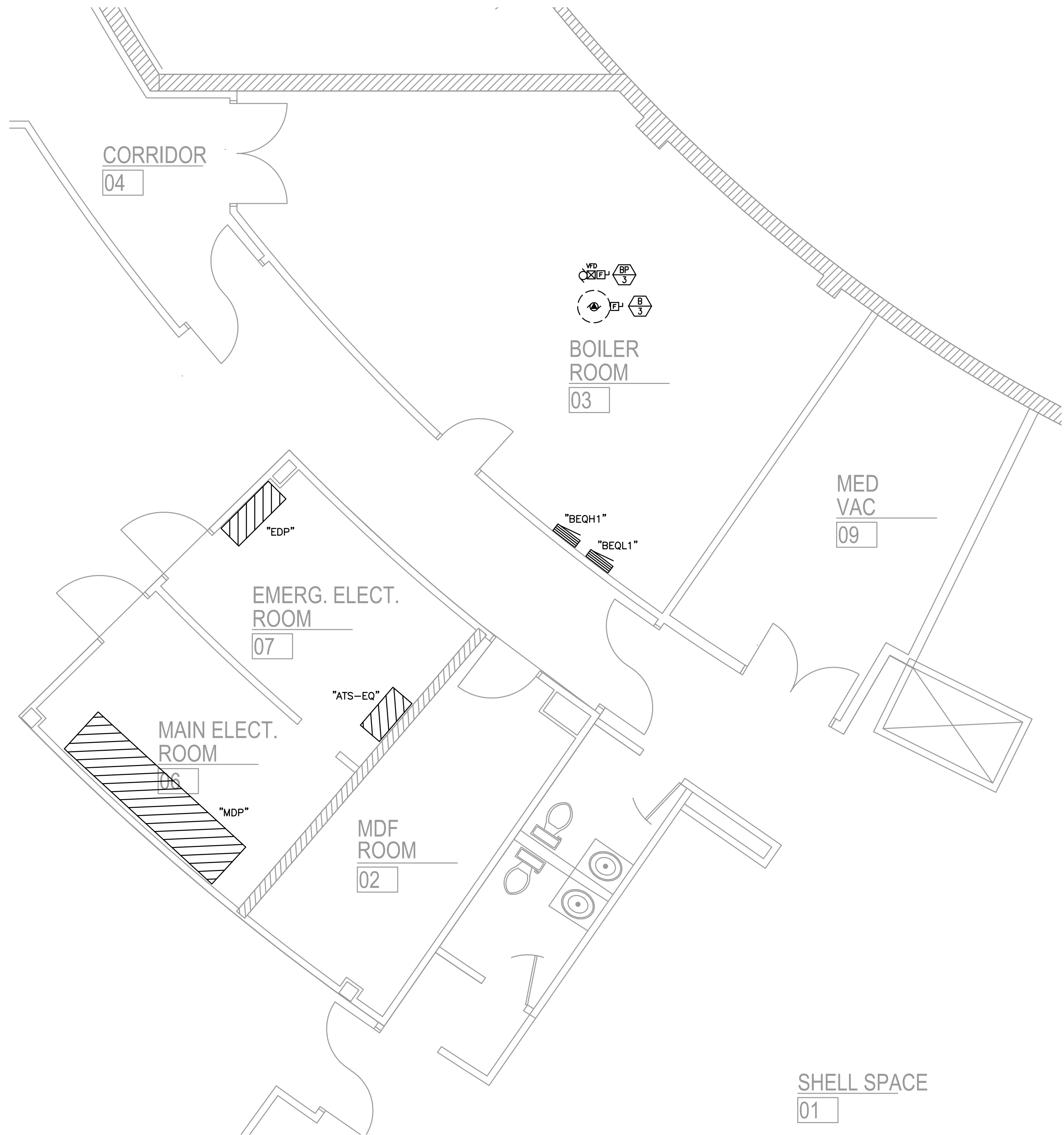
1 BASEMENT ELECTRICAL PLAN E3.4 SCALE: 1/4" = 1'-0"
