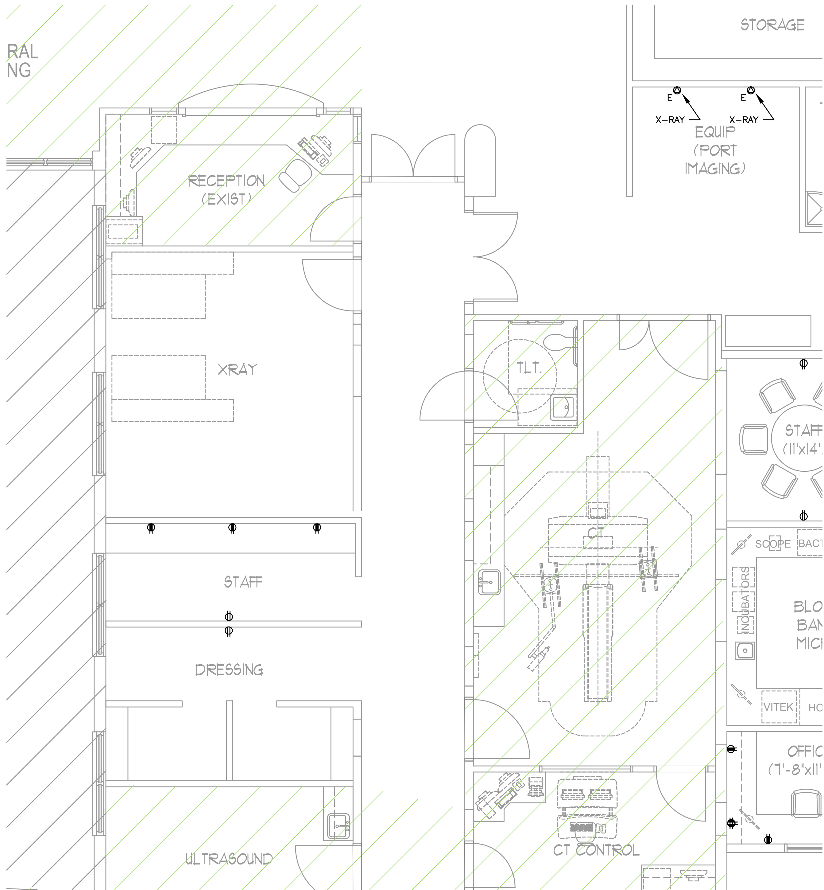
1 POWER PLAN E3.3 SCALE: 1/4" = 1'-0"
