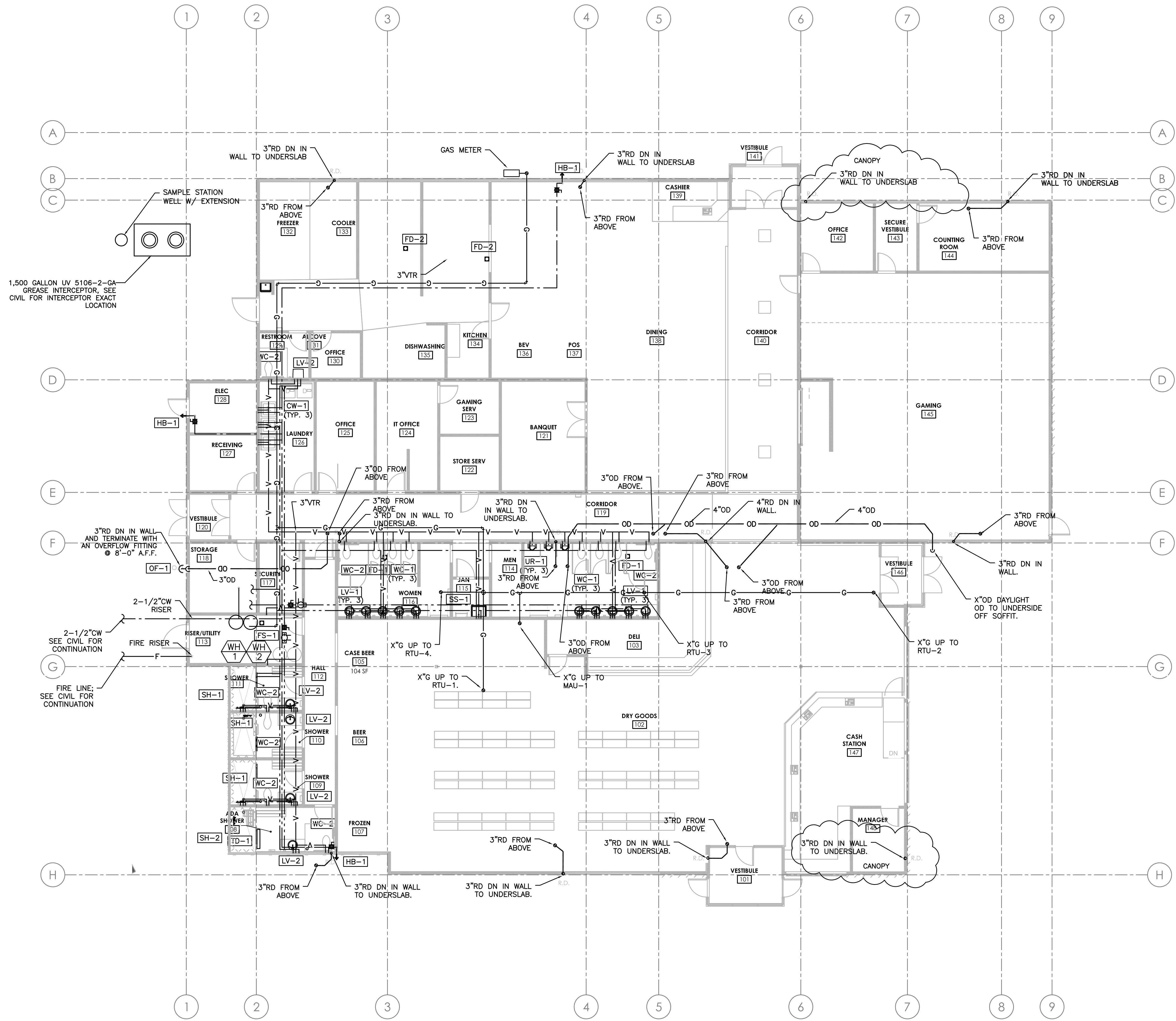
1 PLUMBING FLOOR PLAN SCALE: 1/8"=1'-0"
