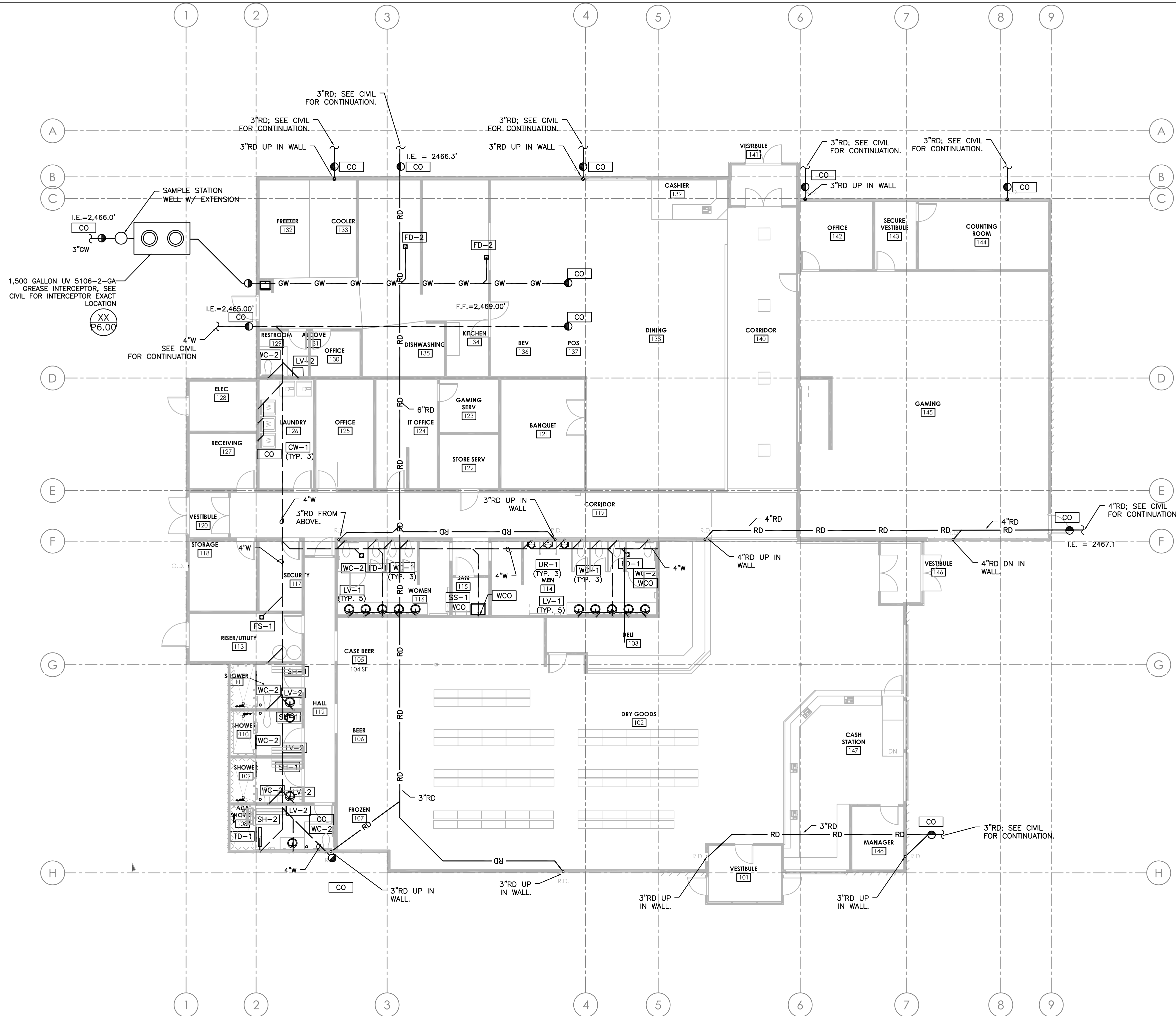
1 UNDER SLAB PLUMBING PLAN P2.01 SCALE: 1/8" = 1'-0"
