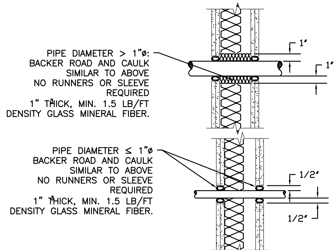
3 PIPE/CONDUIT PENETRATION DRYWALL CONSTRUCTION TO BE APPLIED TO WALLS WITH STC ≥49 SEE ARCHITECTURAL DRAWINGS FOR ACOUSTICALLY IMPORTANT WALLS (WALL TYPES). SEAL PENETRATIONS IN THOSE WALLS PER THESE DETAILS
