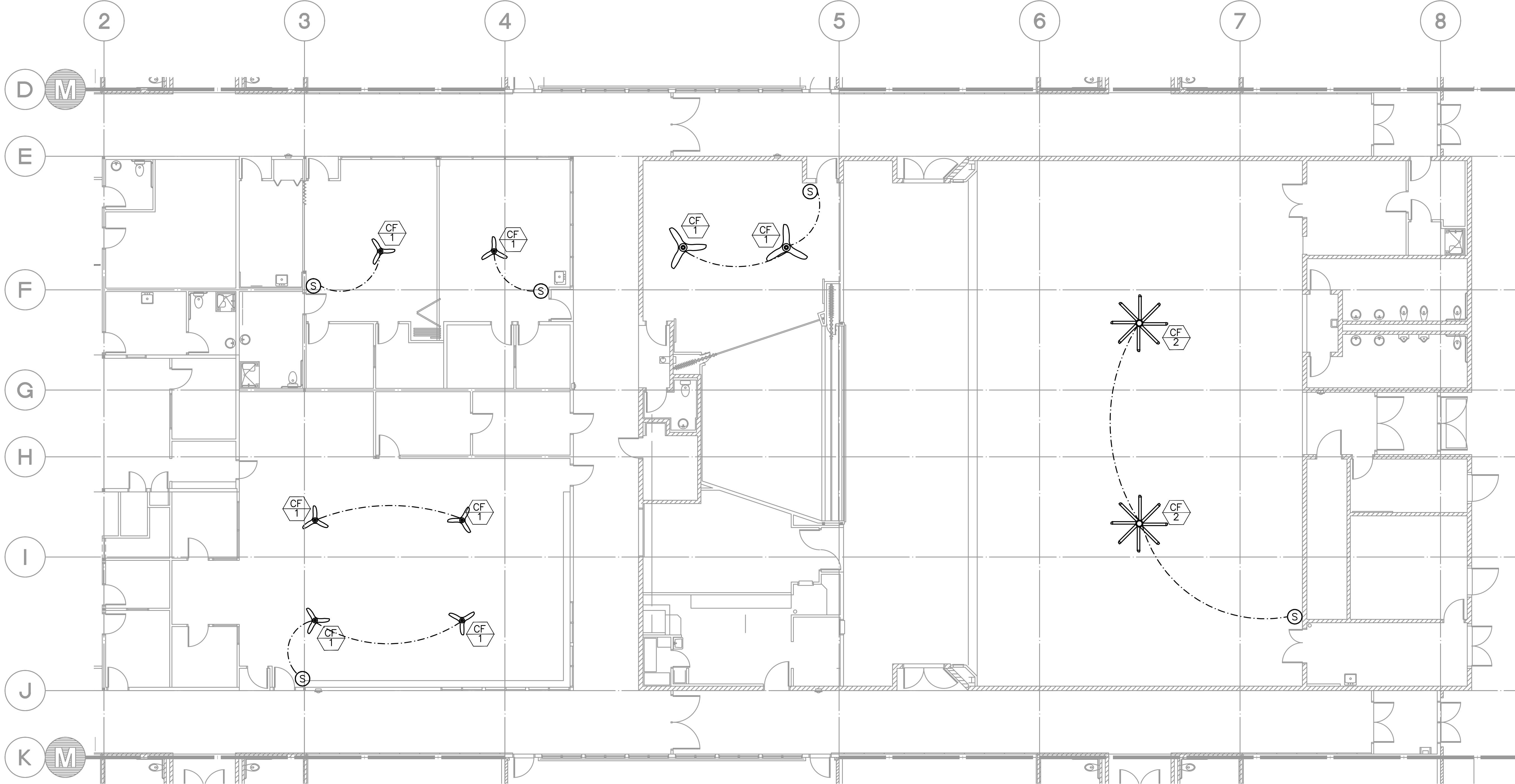
1 HVAC FLOOR PLAN- CENTRAL CORE M1 3 SCALE: 1/8" = 1'-0"
