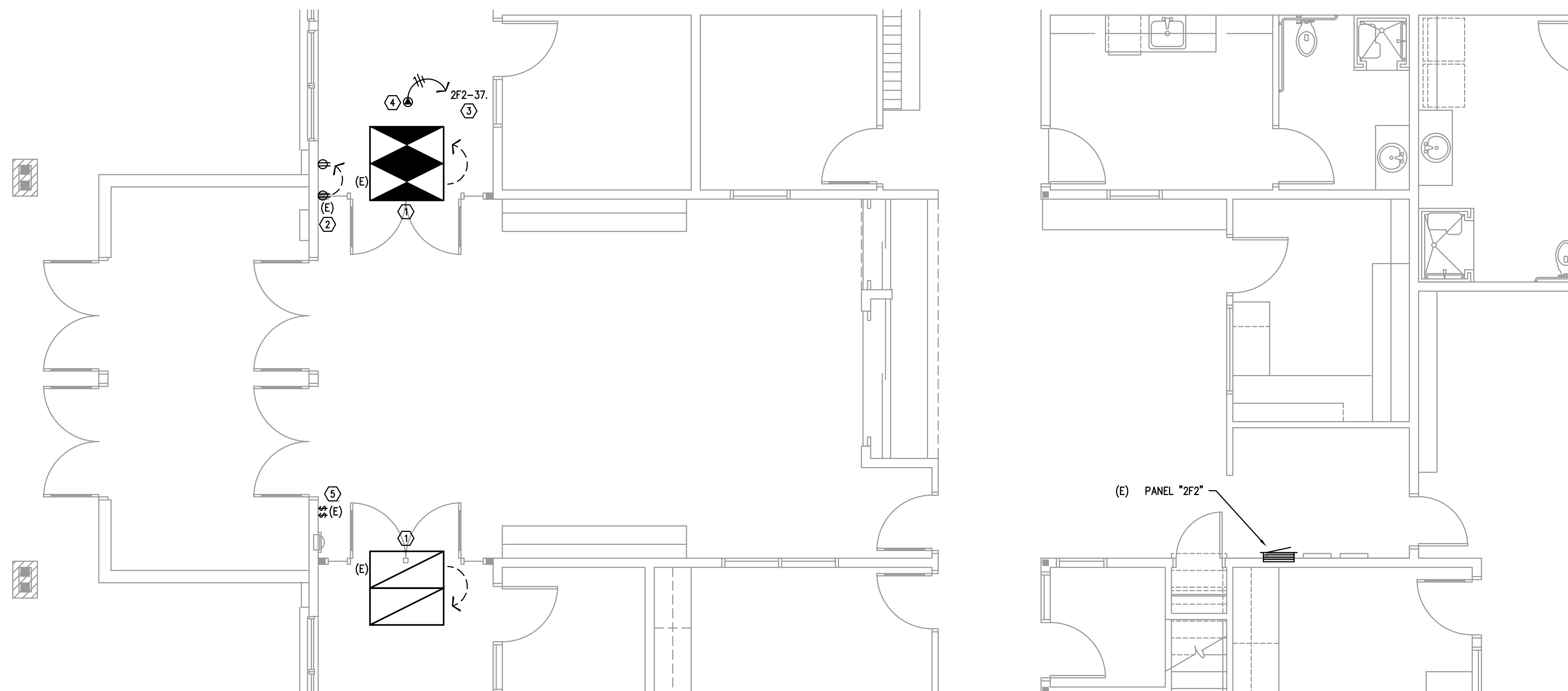
1 ENLARGED FLOOR PLAN - ELECTRICAL E1.1 SCALE: 1/4" = 1'-0"
