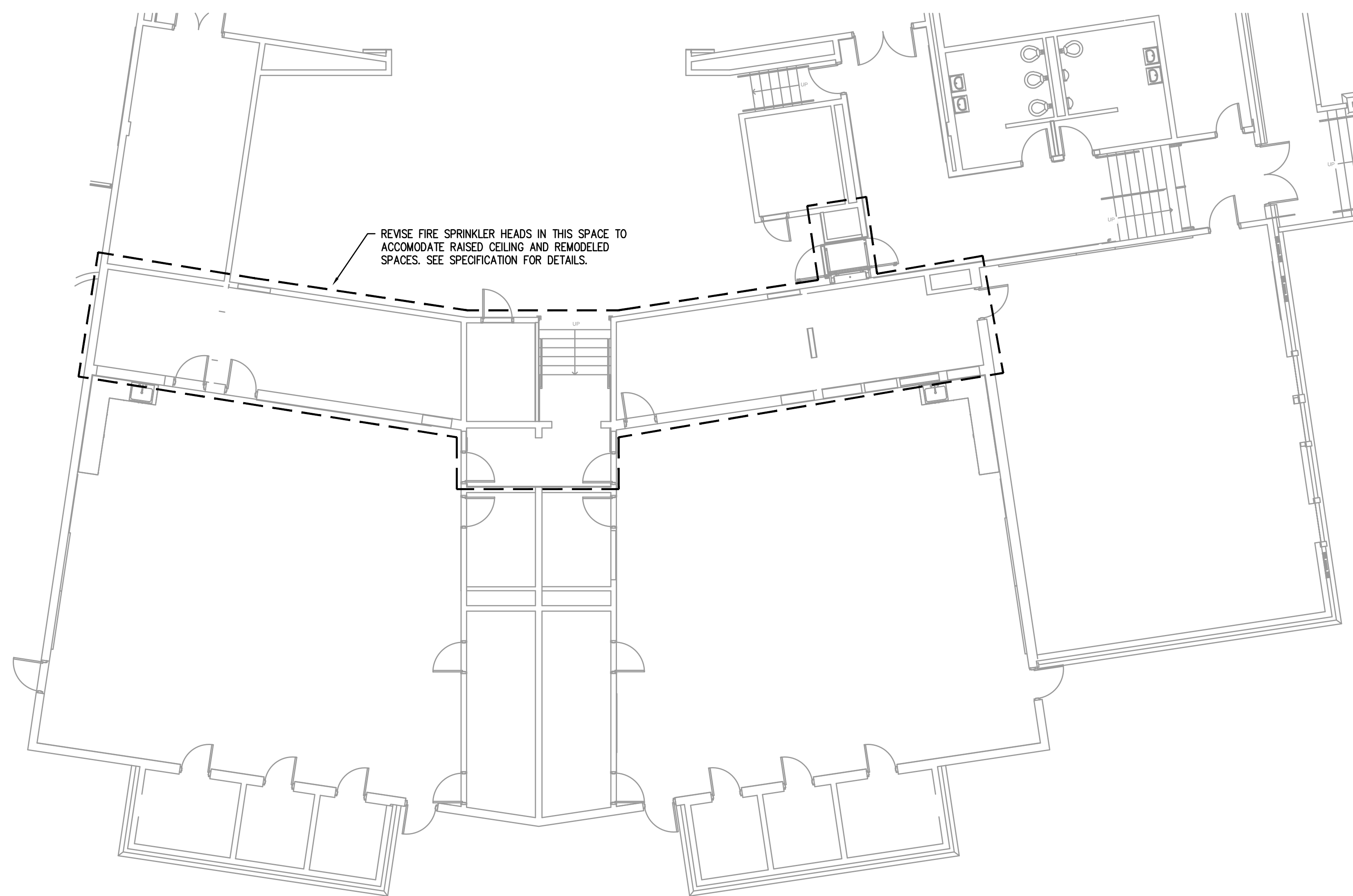
1 FIRE SPRINKLER PLAN FS1.00 SCALE: 1/8"=1'-0"
