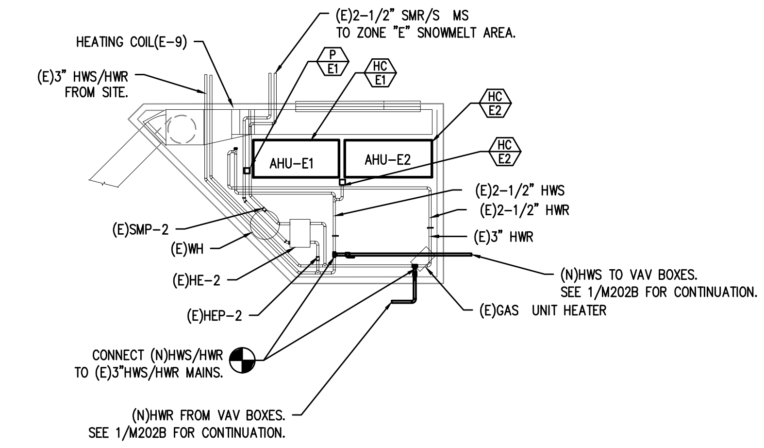
3 MECHANICAL ROOM PIPING DETAIL M2.02B SCALE: 1/8"=1'-0"
