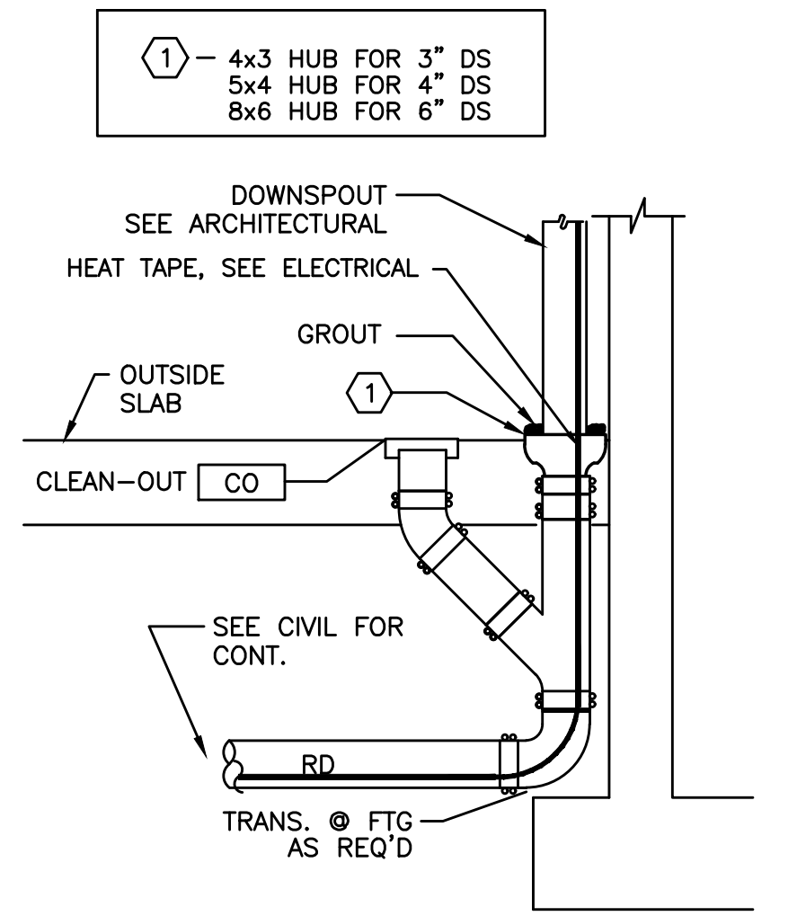
1 DOWN SPOUT DETAIL SCALE: DETAIL
