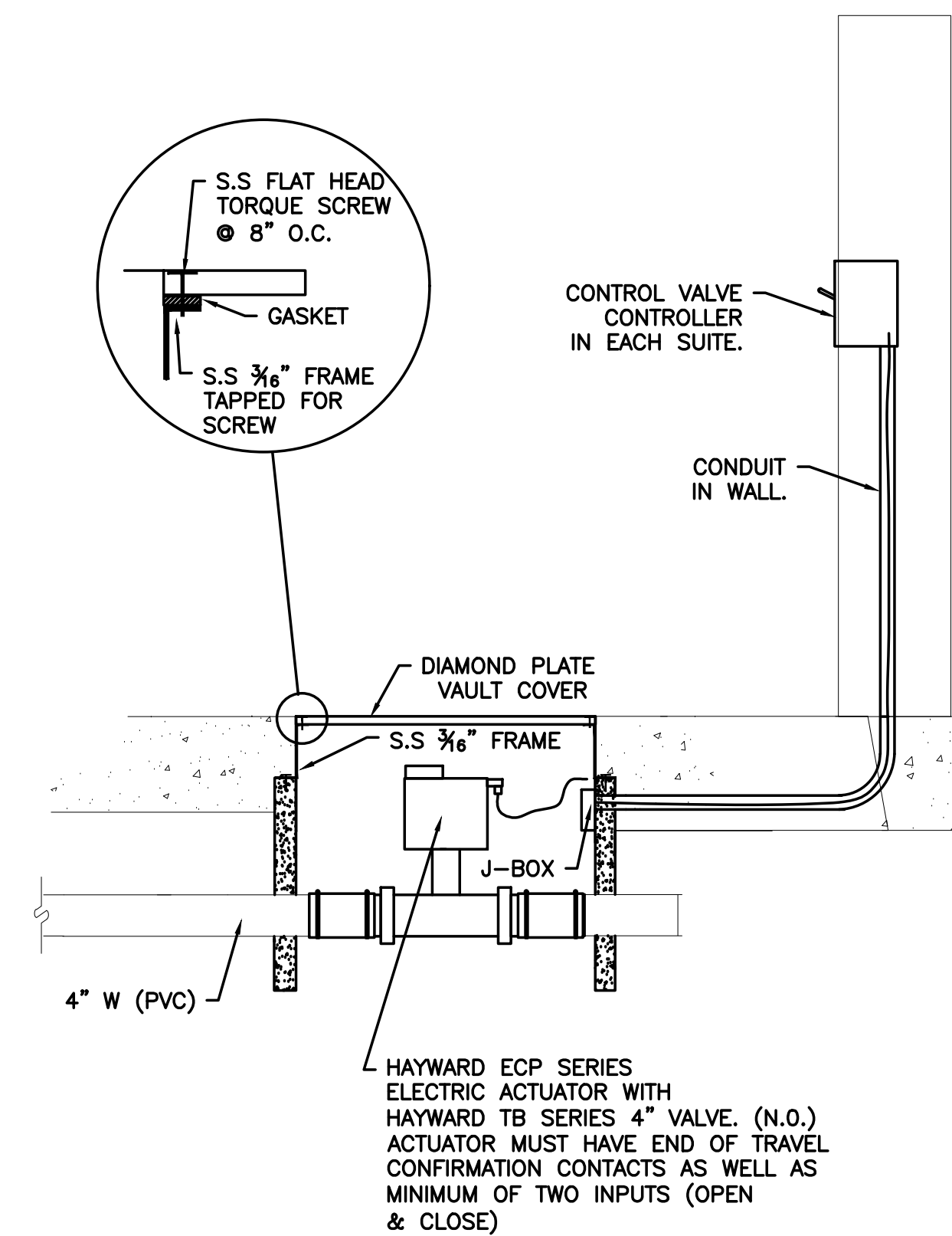
1 SHUT-OFF VALVE INSTALLATION DETAIL P6.1 NO SCALE
