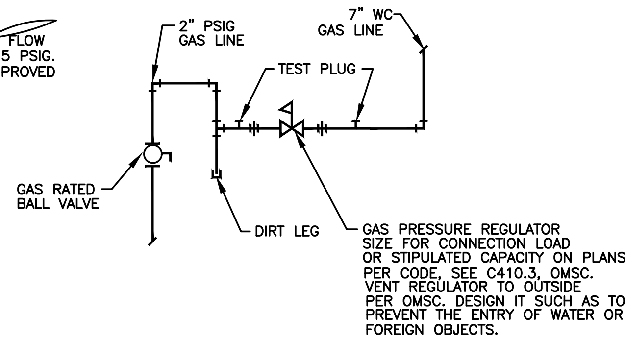
5 CONTROL VALVE CONTROL P6.1 NO SCALE
