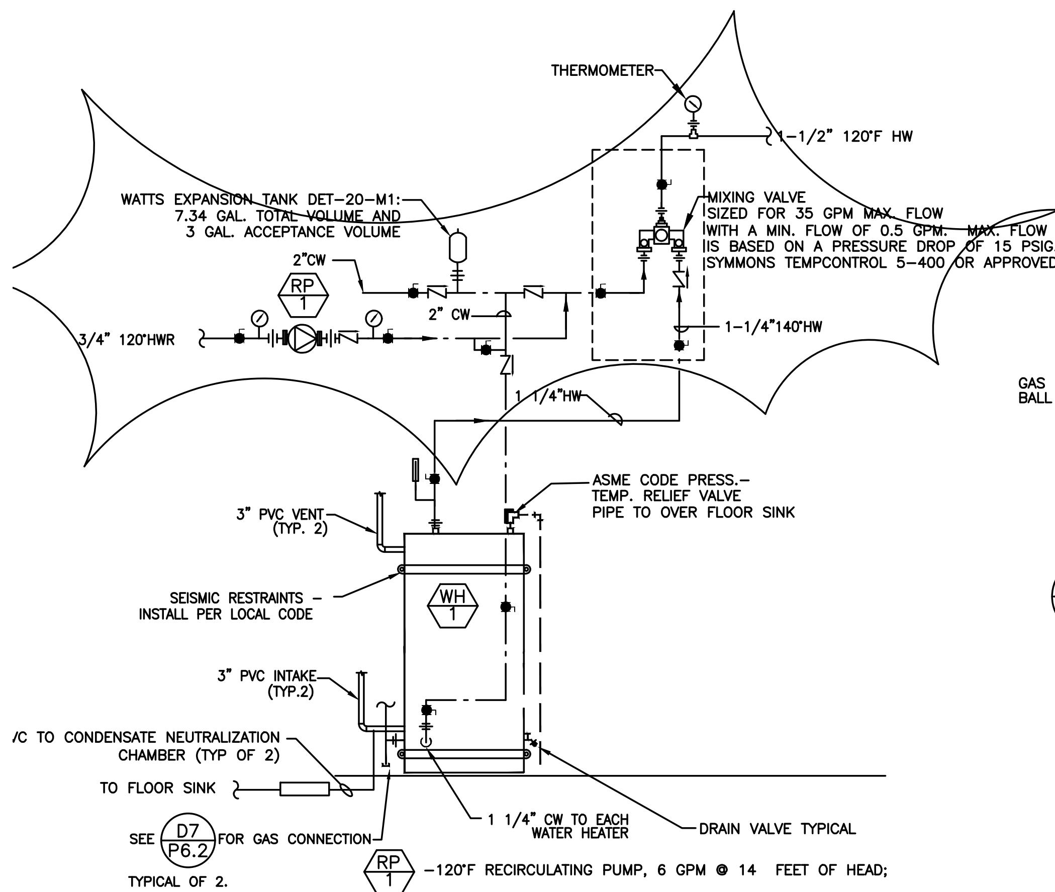
4 HOT WATER HEATER INSTALLATION DETAIL P6.1 NO SCALE
