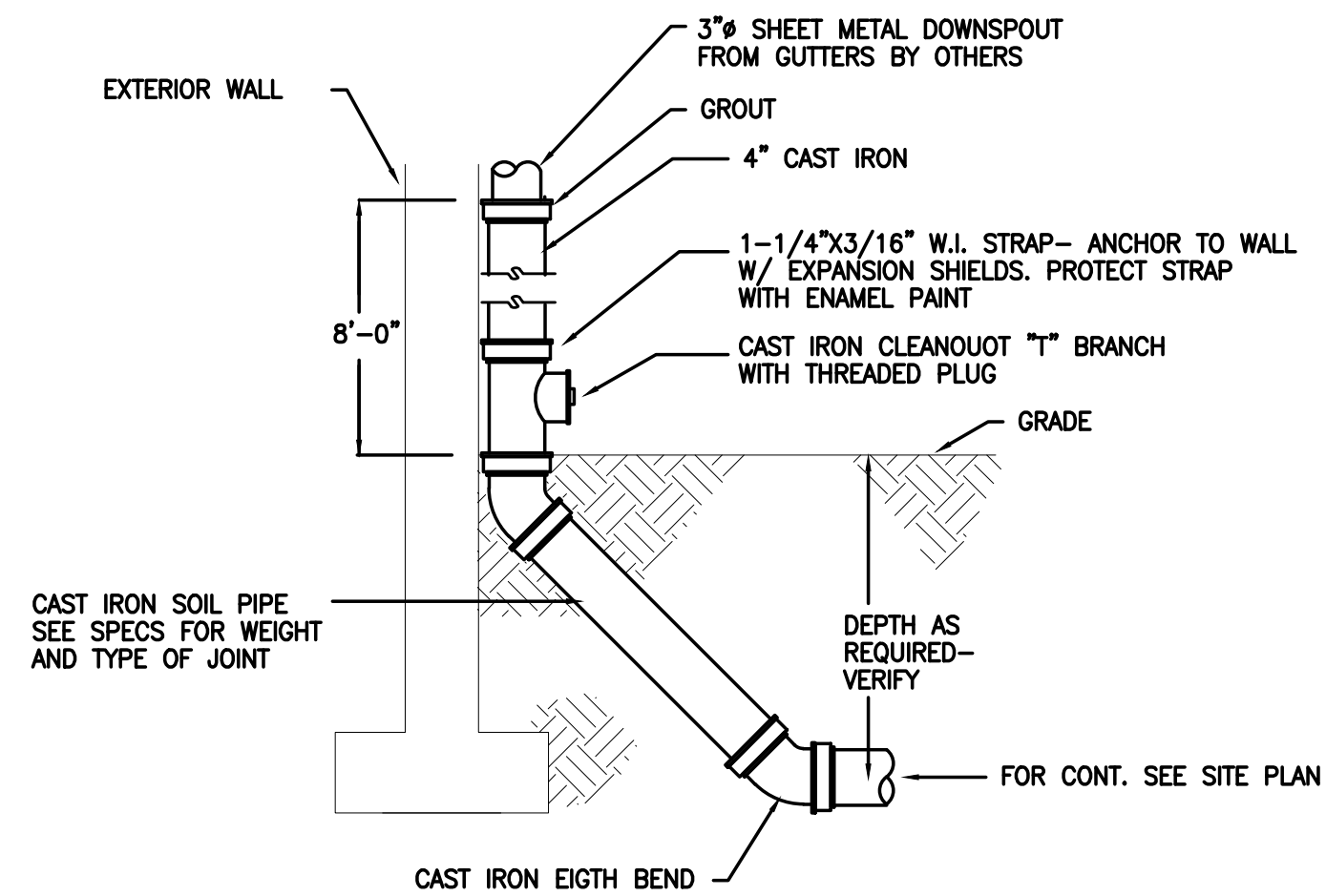
3 DOWNSPOUT CONNECTOIN P6.1 NO SCALE
