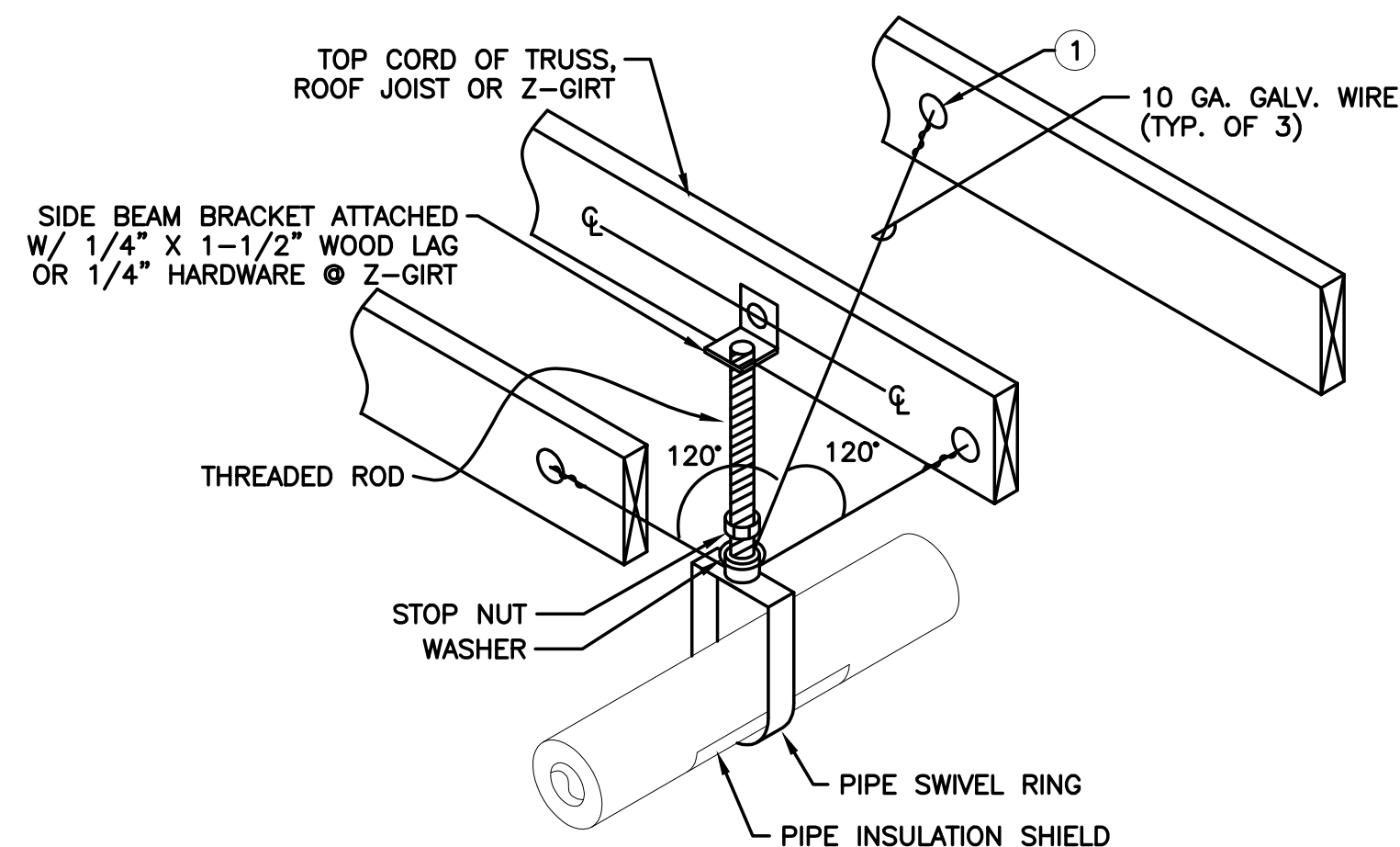
6 NON-SEISMIC PIPE SUPPORT P6.1 NO SCALE
